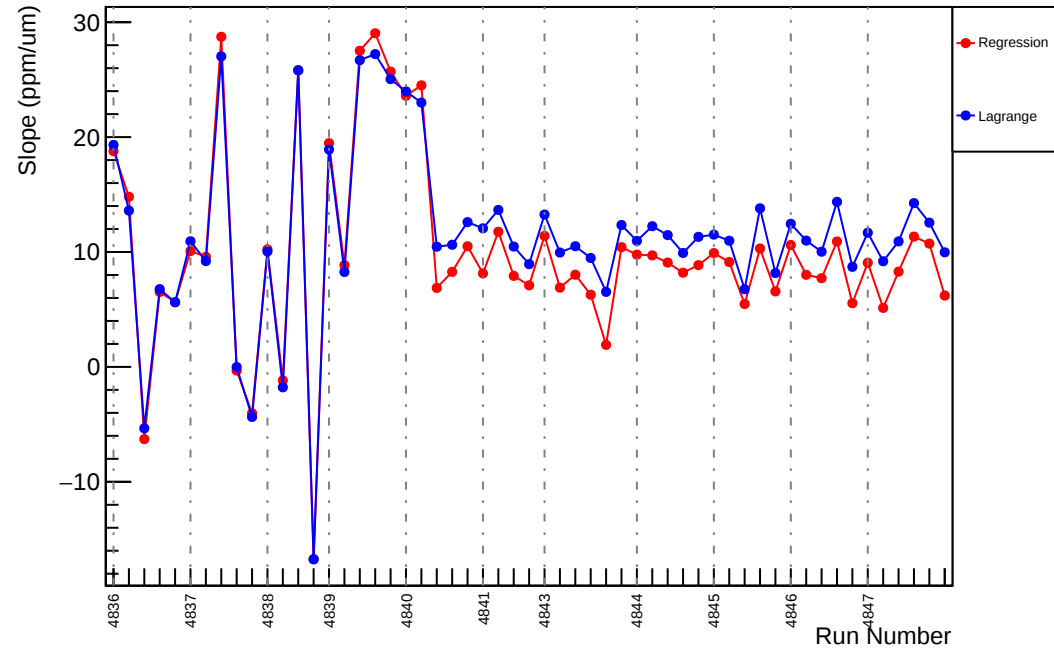
Slug85: Slope : usl_vs_evMon7 (ppm/um)
