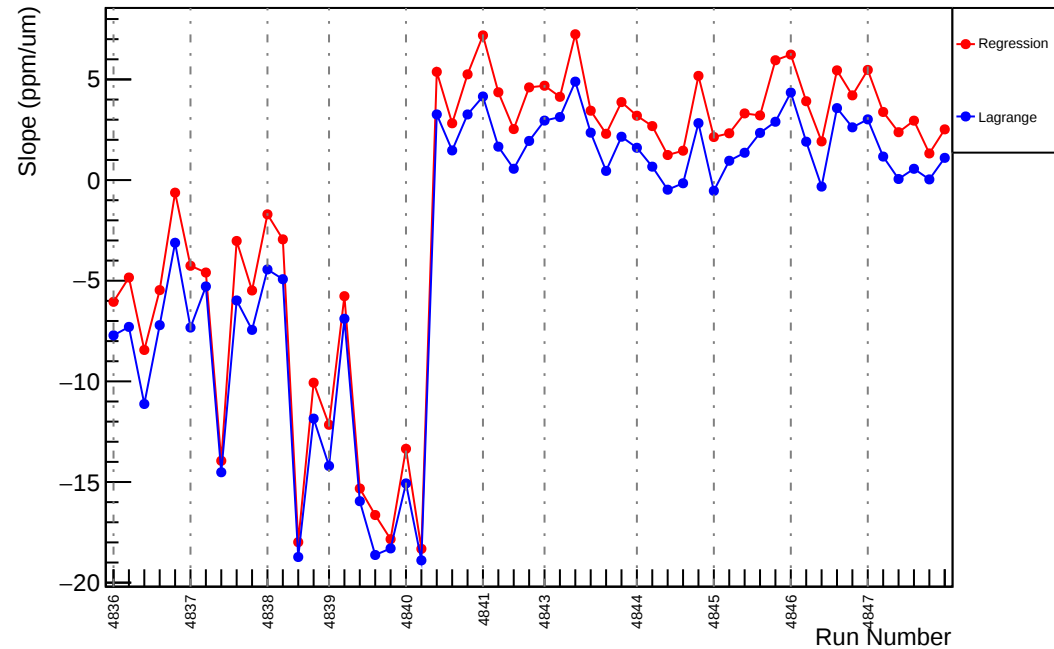
Slug85: Slope : usl_vs_evMon6 (ppm/um)
