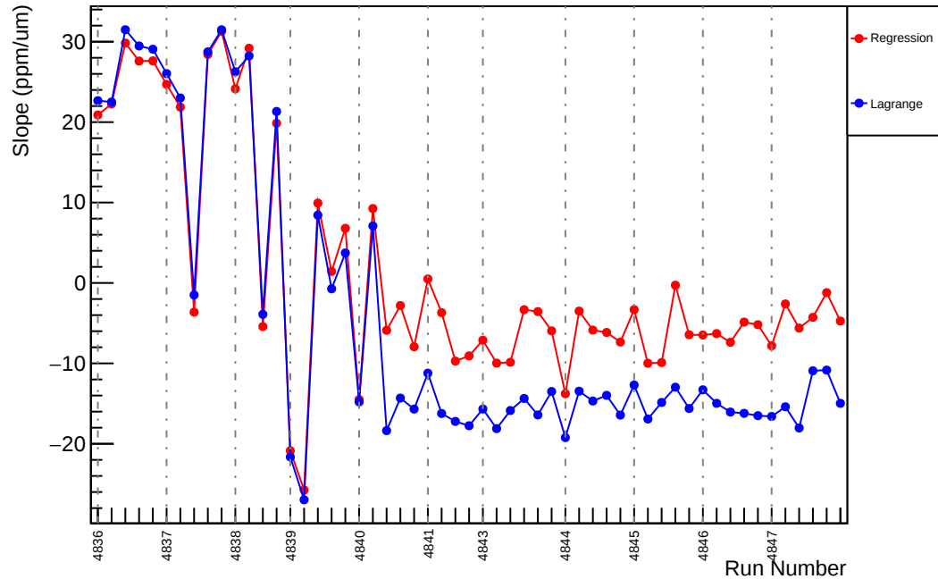
Slug85: Slope : usl_vs_evMon8 (ppm/um)
