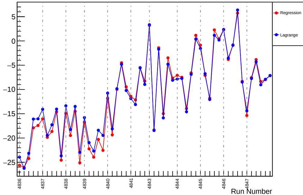
Slug85: Slope : usl_vs_evMon11 (ppm/um)
