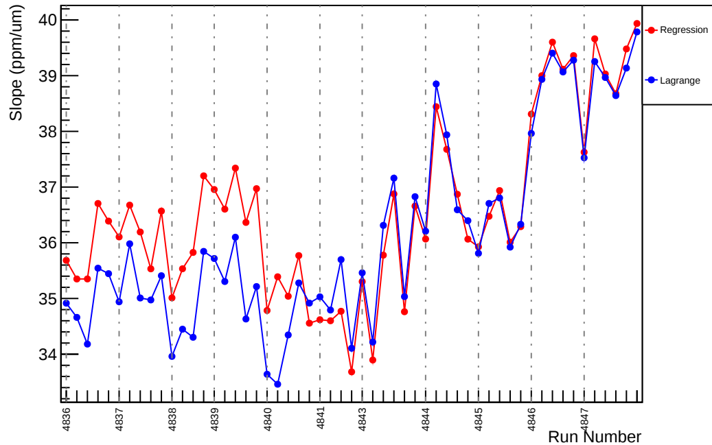
Slug85: Slope : usl_vs_evMon0 (ppm/um)
