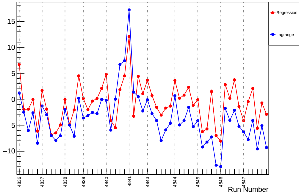
Slug85: Slope : usl_vs_evMon9 (ppm/um)
