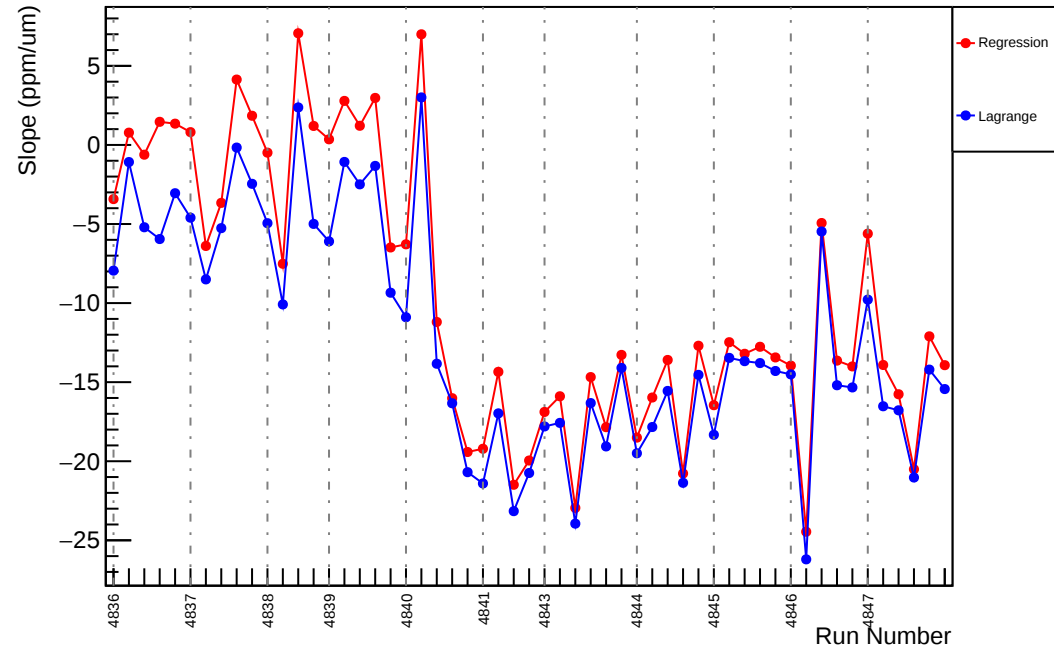
Slug85: Slope : usl_vs_evMon10 (ppm/um)
