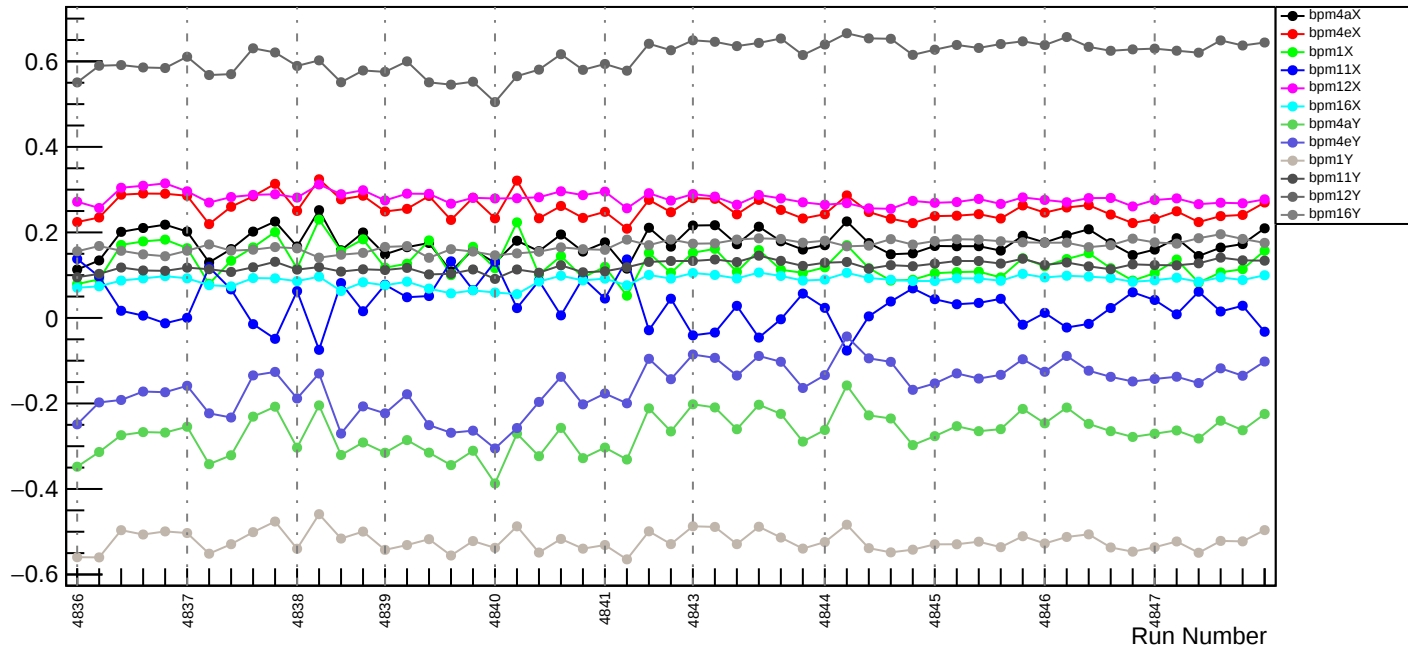
Slug85: EigenVector #3
