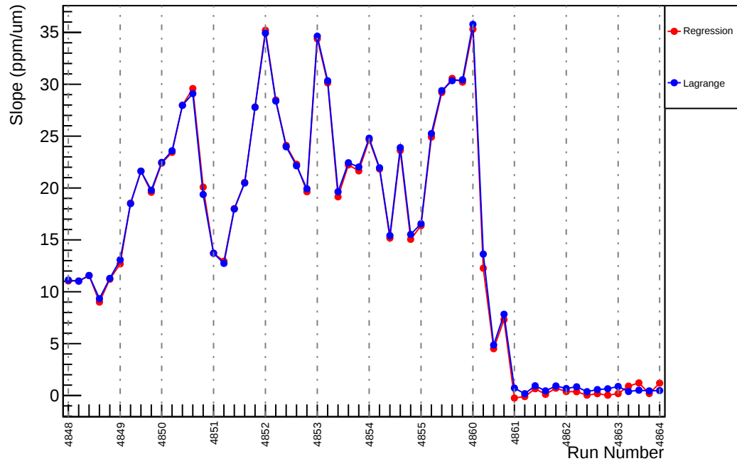
Slug86: Slope : us_avg_vs_evMon0 (ppm/um)
