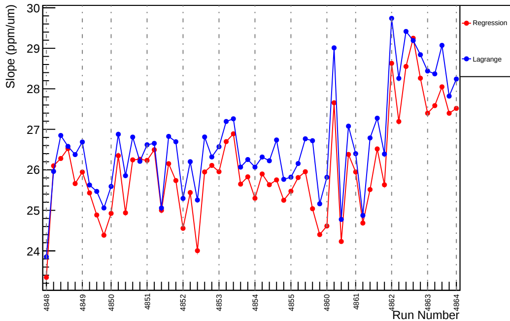
Slug86: Slope : us_avg_vs_evMon2 (ppm/um)
