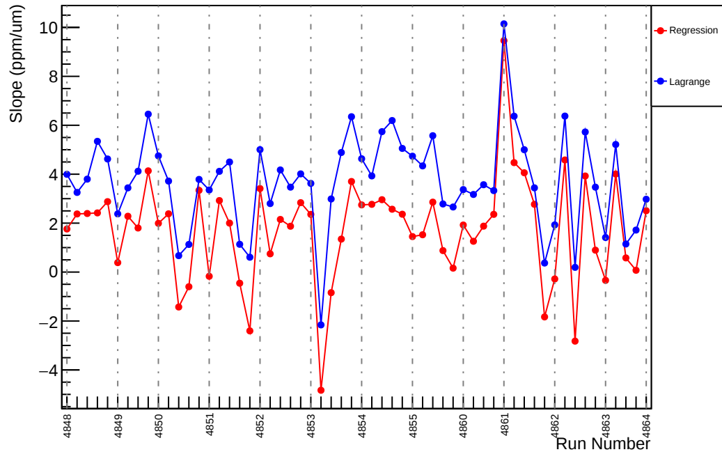
Slug86: Slope : us_avg_vs_evMon7 (ppm/um)
