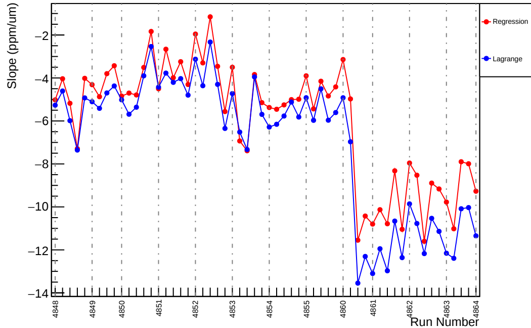
Slug86: Slope : us_avg_vs_evMon5 (ppm/um)
