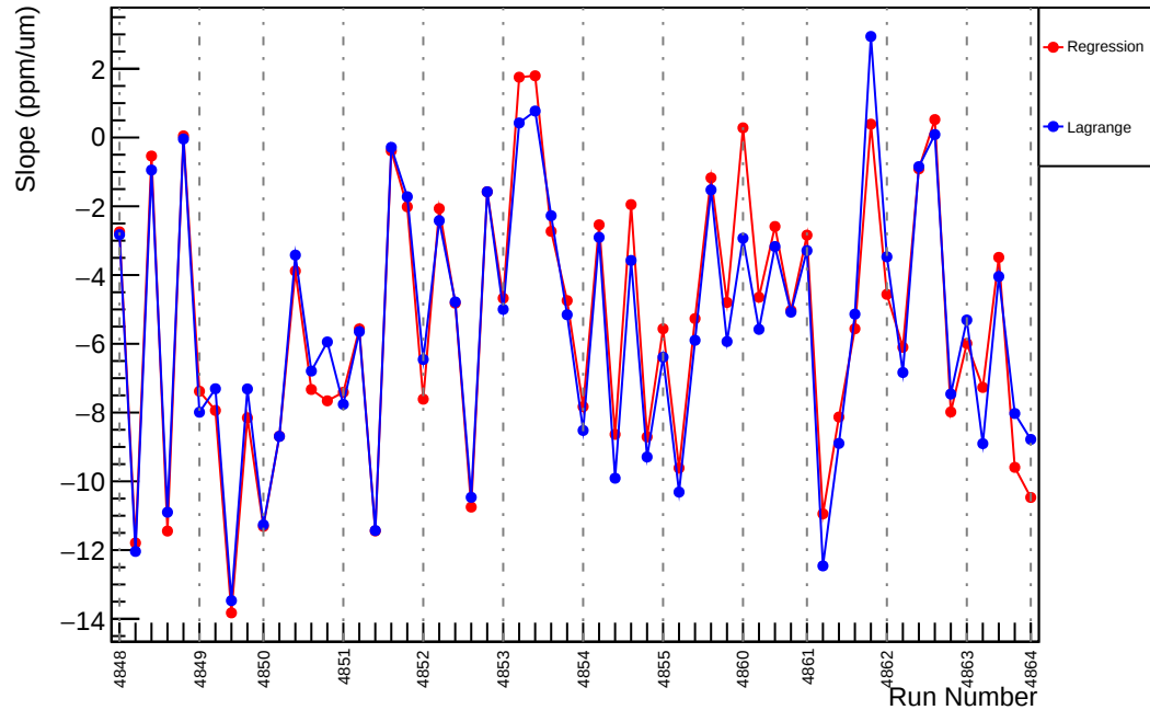
Slug86: Slope : us_avg_vs_evMon11 (ppm/um)
