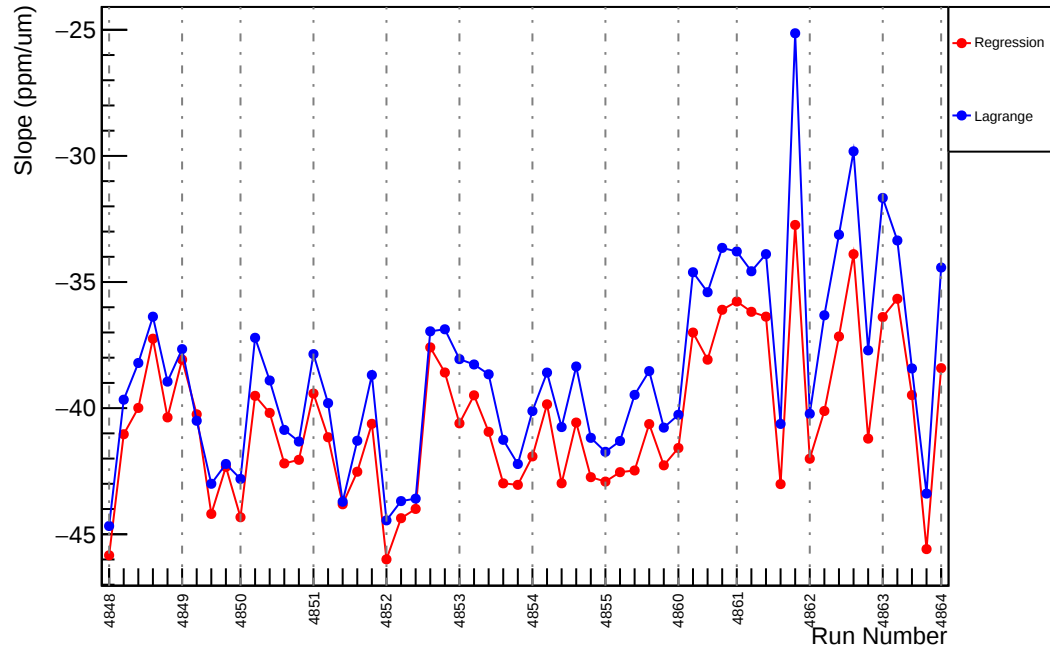
Slug86: Slope : us_dd_vs_evMon4 (ppm/um)
