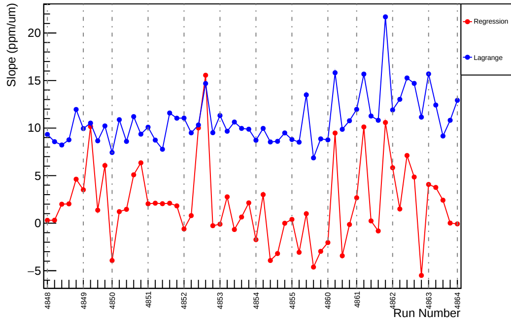
Slug86: Slope : us_dd_vs_evMon5 (ppm/um)
