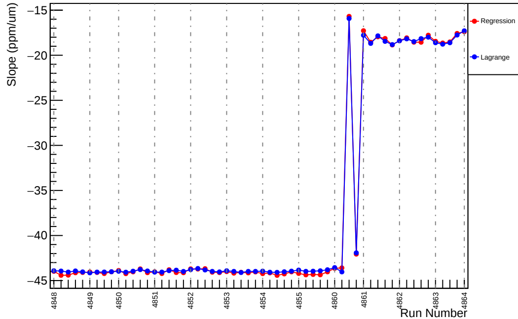
Slug86: Slope : us_dd_vs_evMon1 (ppm/um)
