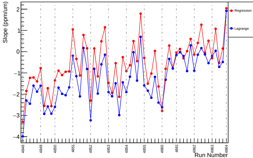
Slug86: Slope : us_dd_vs_evMon2 (ppm/um)
