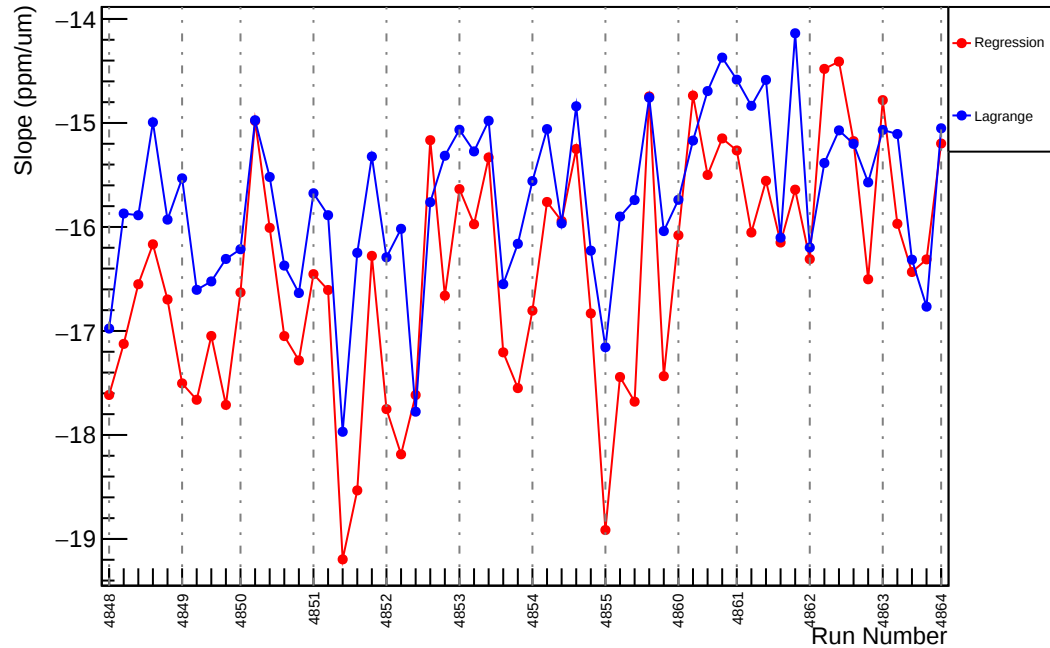
Slug86: Slope : us_dd_vs_evMon3 (ppm/um)
