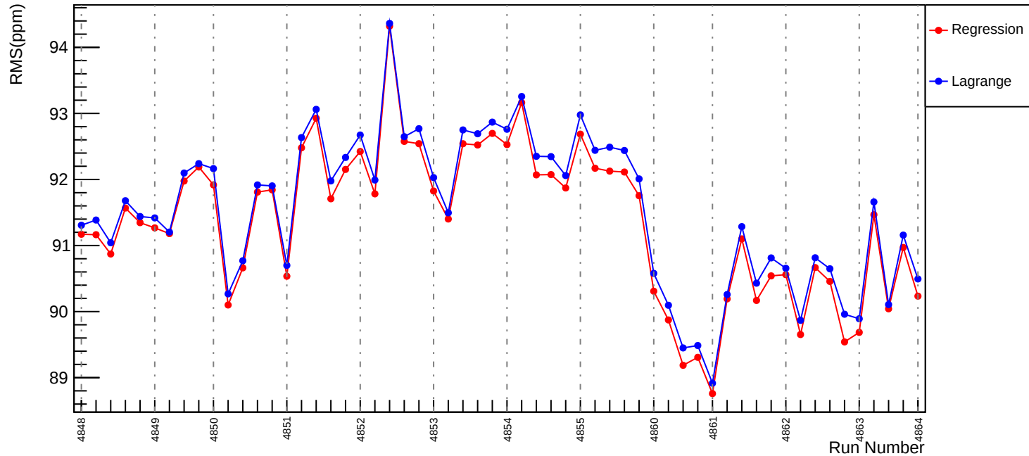
Slug86: Corrected RMS (ppm): asym_us_dd
