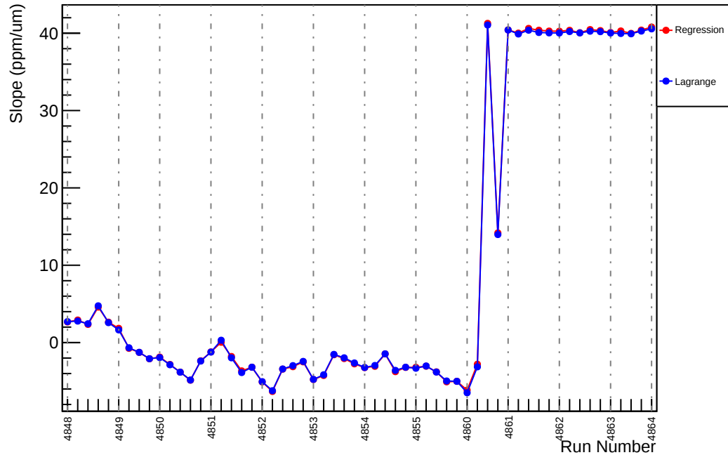
Slug86: Slope : us_dd_vs_evMon0 (ppm/um)
