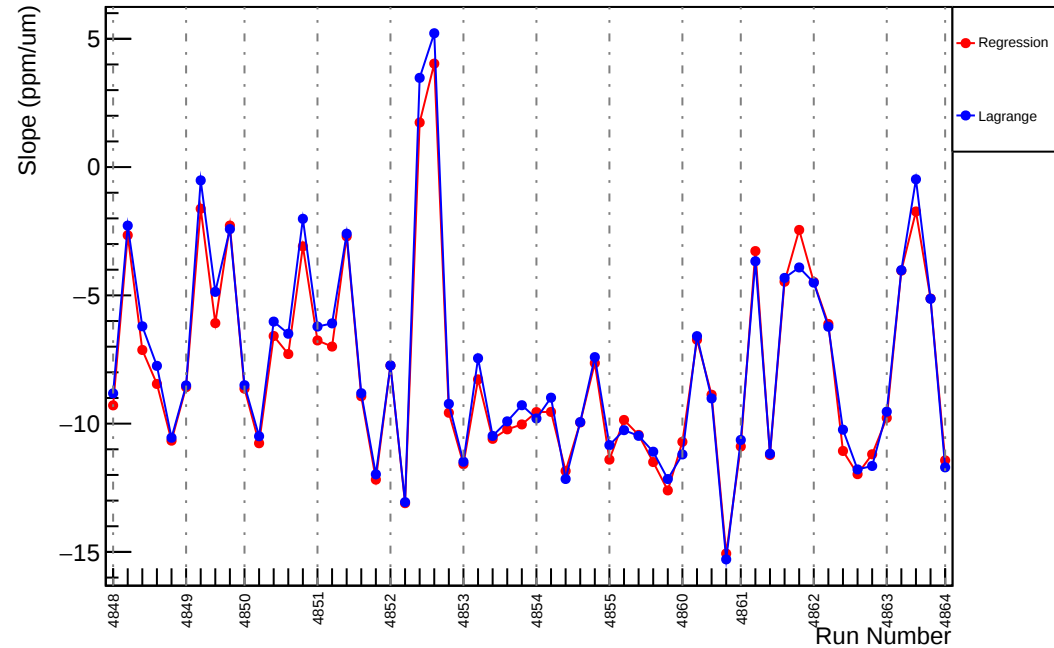
Slug86: Slope : us_dd_vs_evMon10 (ppm/um)
