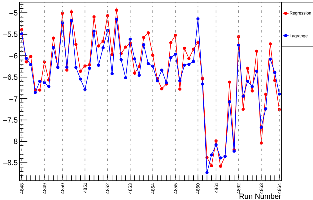
Slug86: Slope : us_dd_vs_evMon2 (ppm/um)
