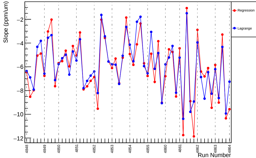
Slug86: Slope : us_dd_vs_evMon9 (ppm/um)
