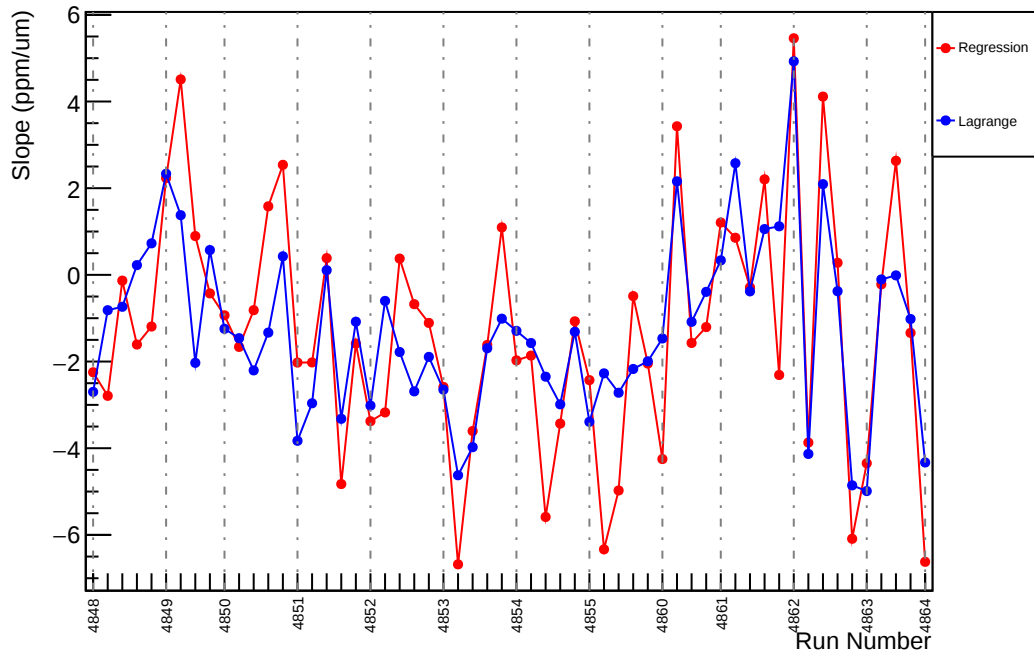
Slug86: Slope : us_dd_vs_evMon8 (ppm/um)
