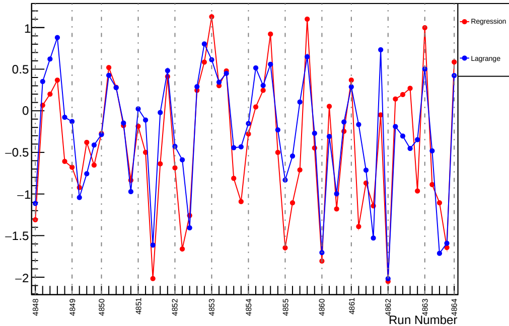
Slug86: Slope : us_dd_vs_evMon4 (ppm/um)
