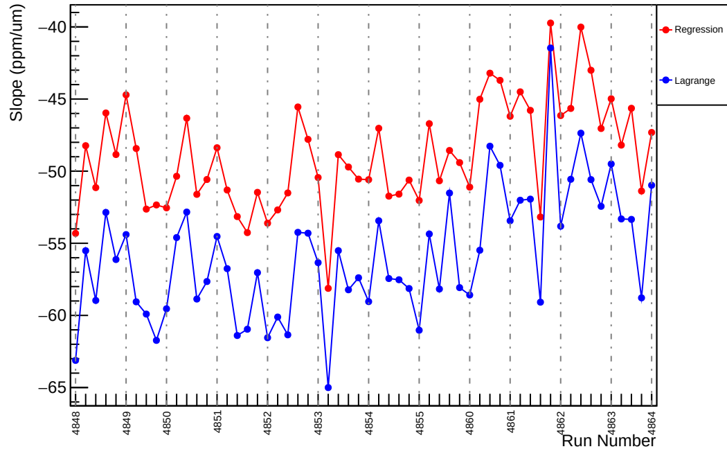
Slug86: Slope : usl_vs_evMon4 (ppm/um)
