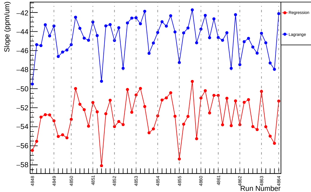
Slug86: Slope : usl_vs_evMon3 (ppm/um)
