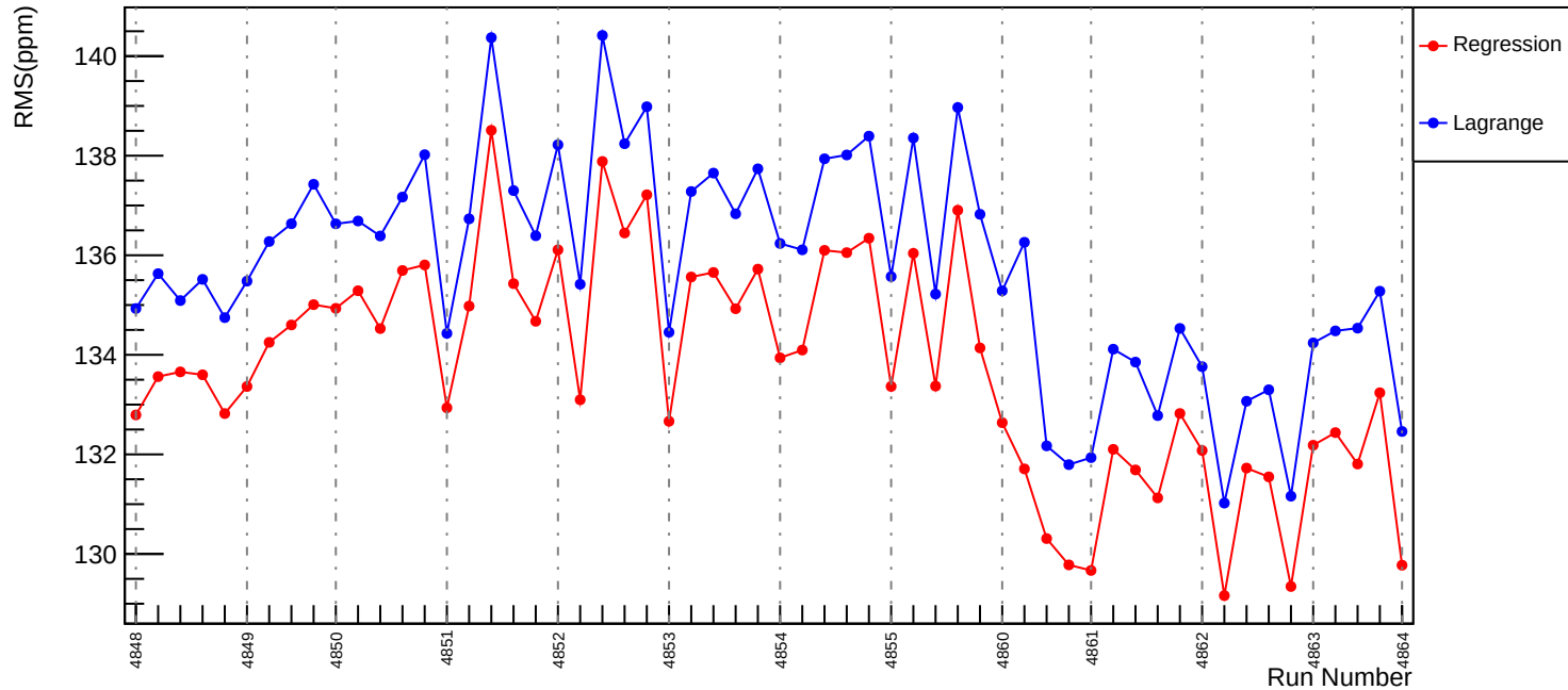
Slug86: Corrected RMS (ppm): asym_usl
