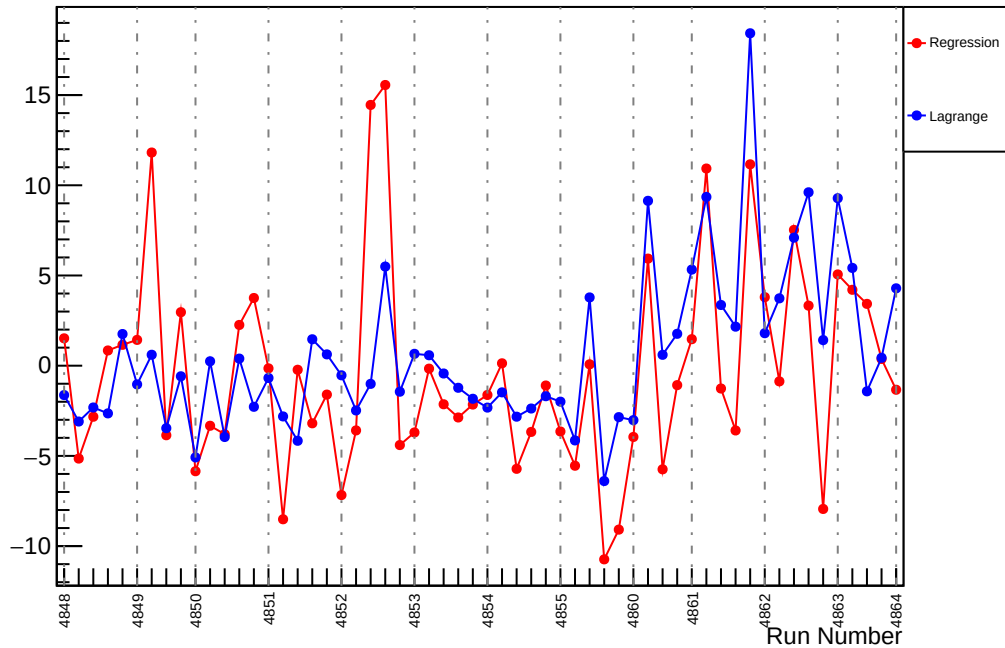
Slug86: Slope : usl_vs_evMon5 (ppm/um)
