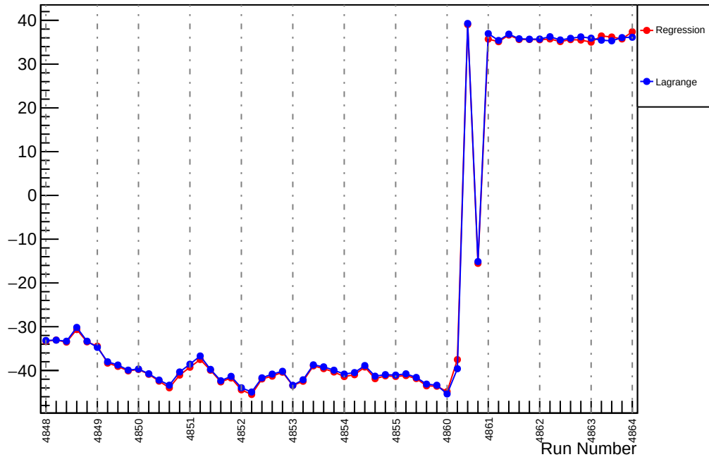
Slug86: Slope : usl_vs_evMon0 (ppm/um)
