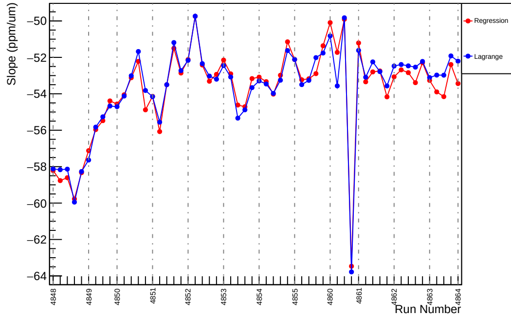
Slug86: Slope : usl_vs_evMon1 (ppm/um)
