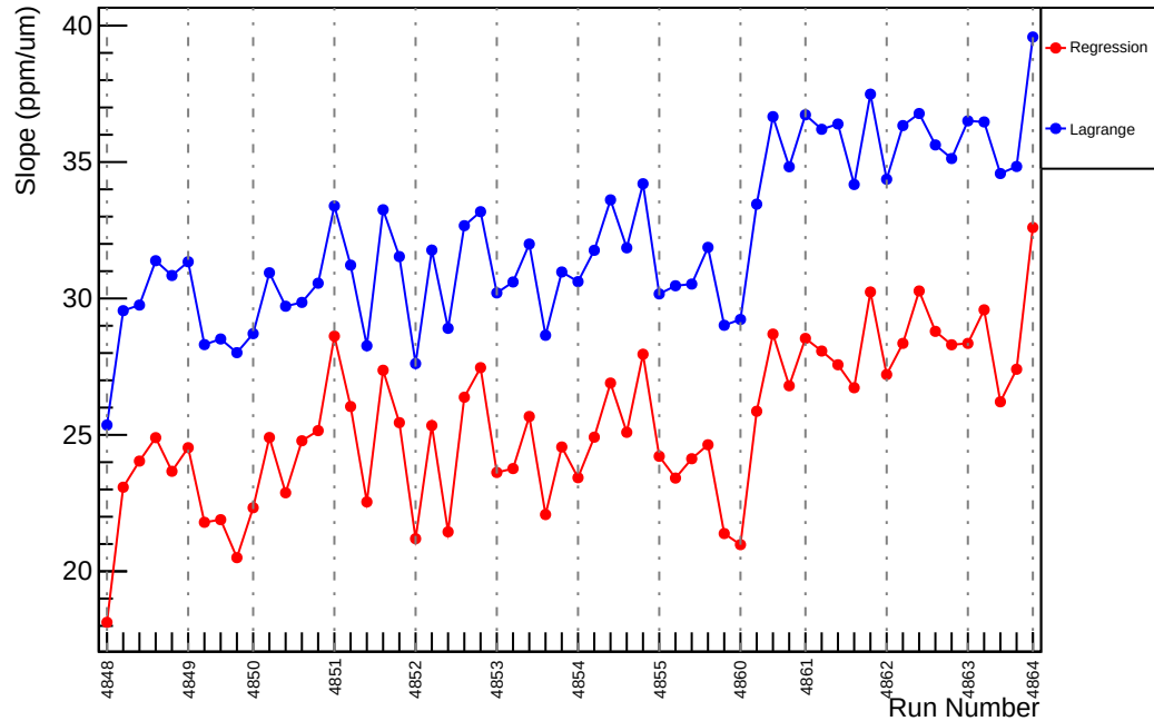
Slug86: Slope : usl_vs_evMon2 (ppm/um)
