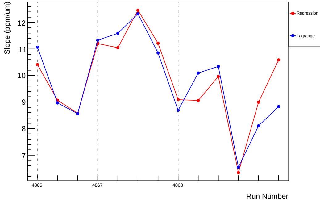
Slug87: Slope : us_avg_vs_evMon6 (ppm/um)
