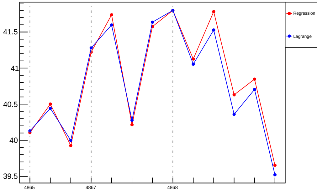
Slug87: Slope : us_dd_vs_evMon0 (ppm/um)
