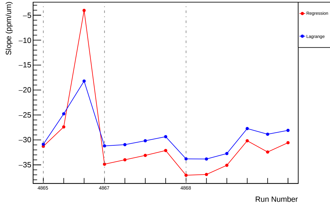
Slug87: Slope : us_dd_vs_evMon4 (ppm/um)
