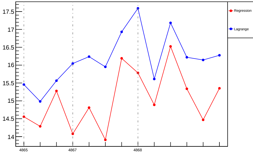
Slug87: Slope : us_dd_vs_evMon3 (ppm/um)
