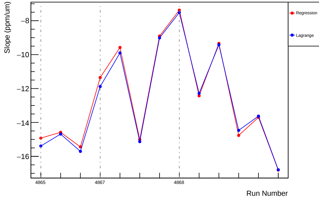
Slug87: Slope : us_dd_vs_evMon1 (ppm/um)
