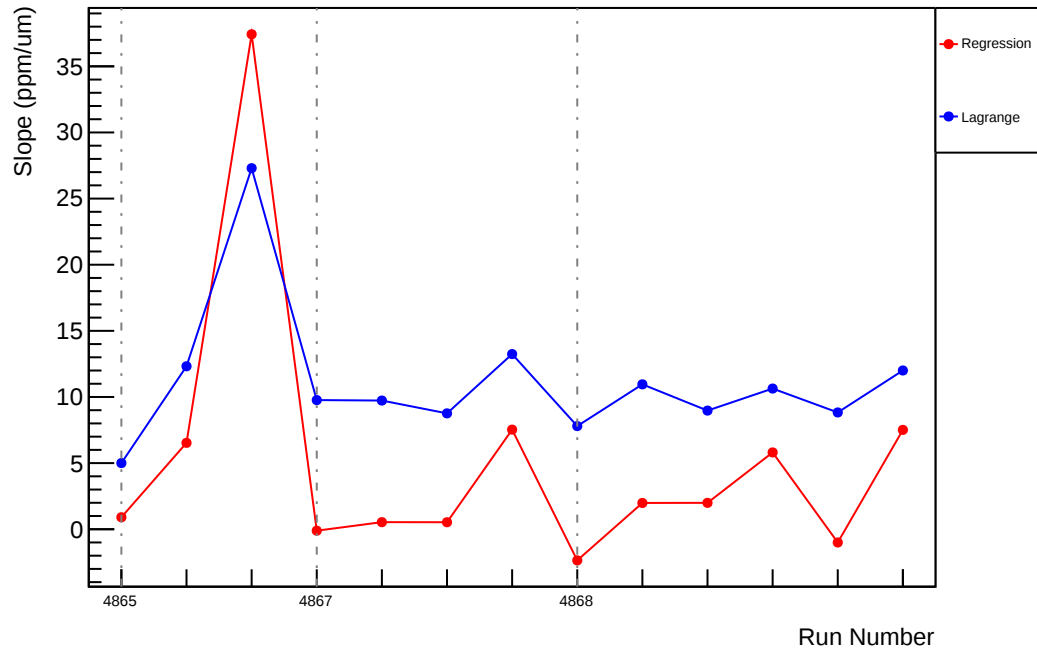
Slug87: Slope : us_dd_vs_evMon5 (ppm/um)
