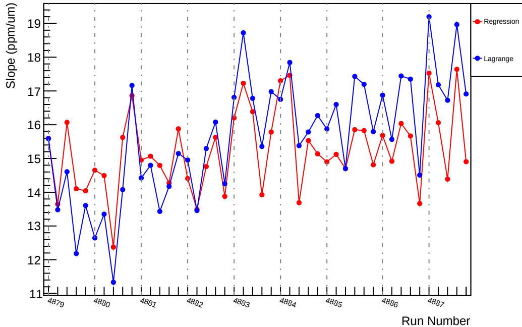
Slug89: Slope : us_avg_vs_evMon6 (ppm/um)
