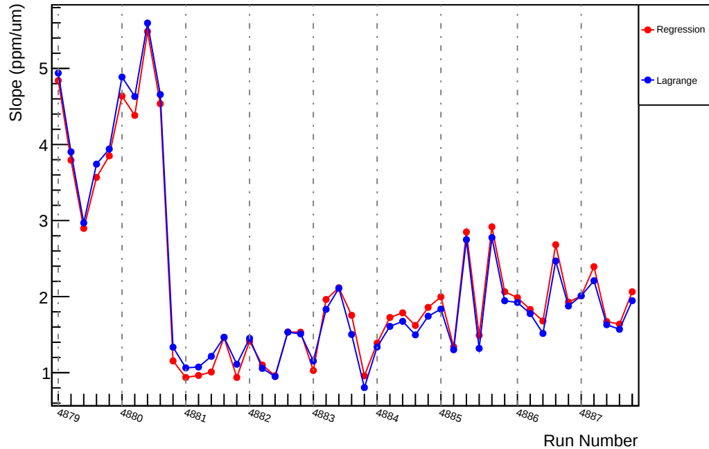
Slug89: Slope : us_avg_vs_evMon0 (ppm/um)
