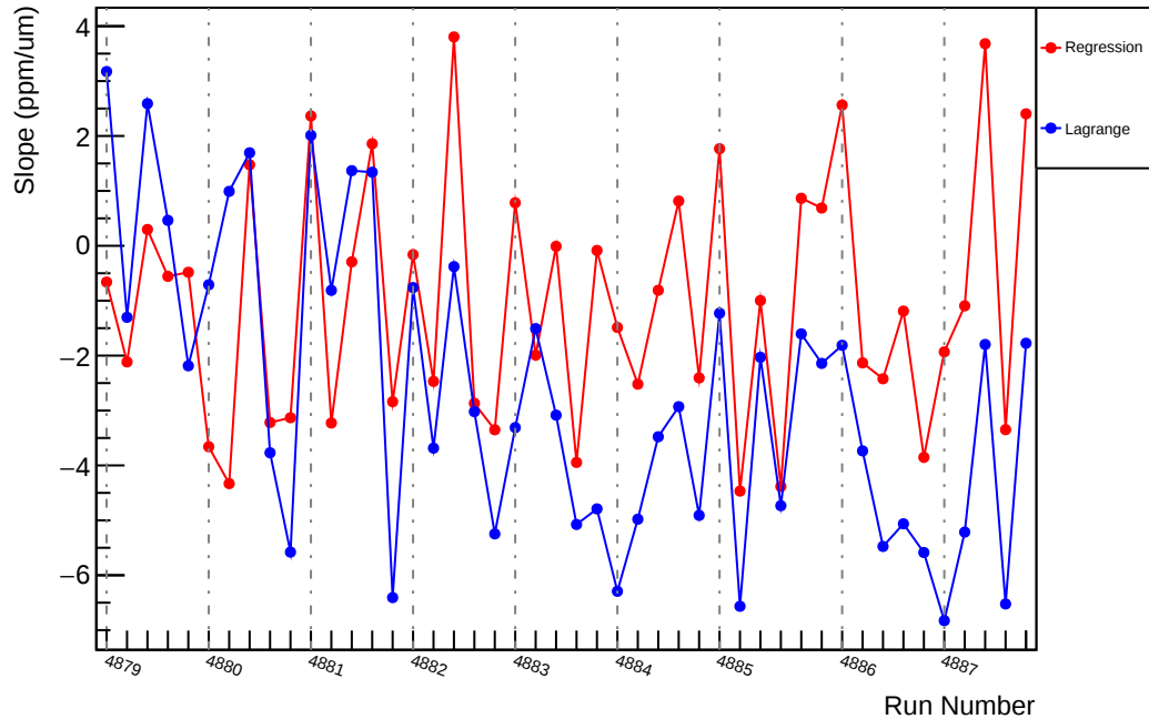
Slug89: Slope : us_avg_vs_evMon9 (ppm/um)
