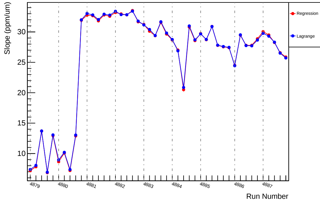
Slug89: Slope : us_dd_vs_evMon0 (ppm/um)
