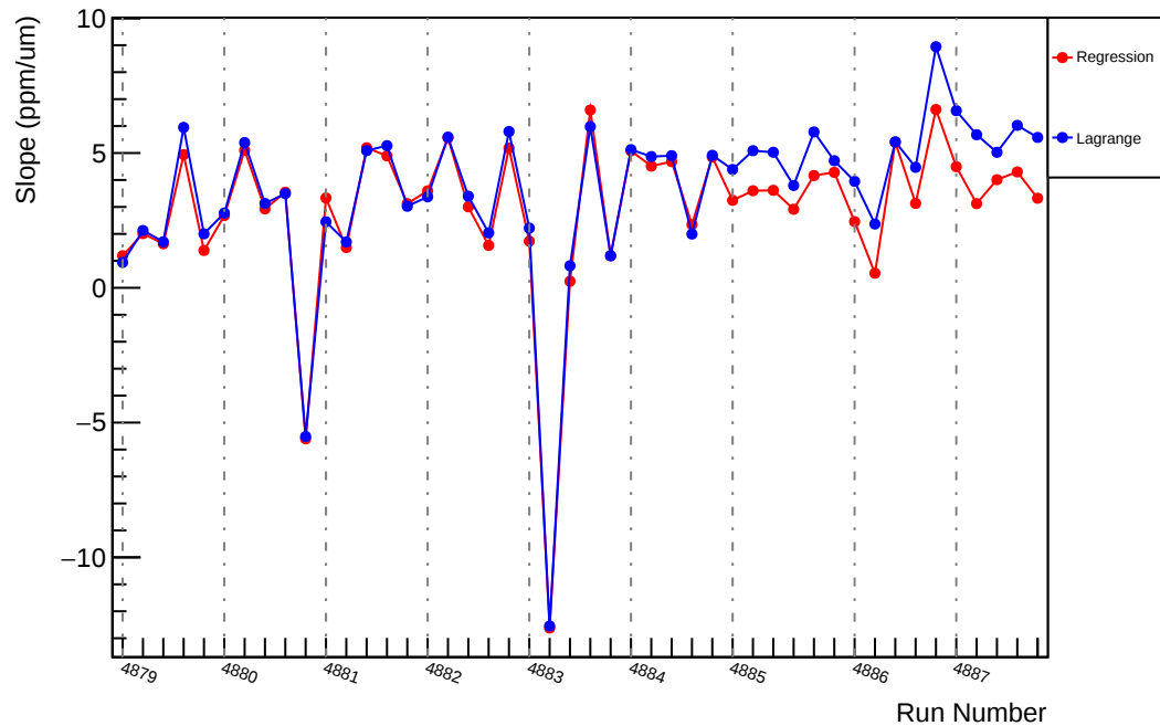
Slug89: Slope : us_dd_vs_evMon6 (ppm/um)
