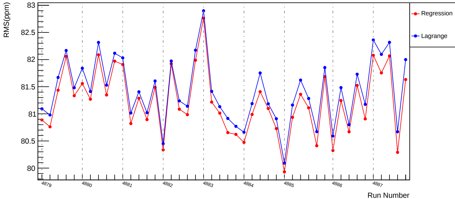
Slug89: Corrected RMS (ppm): asym_us_dd
