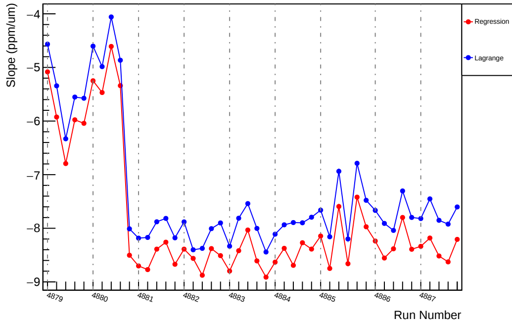
Slug89: Slope : us_dd_vs_evMon1 (ppm/um)
