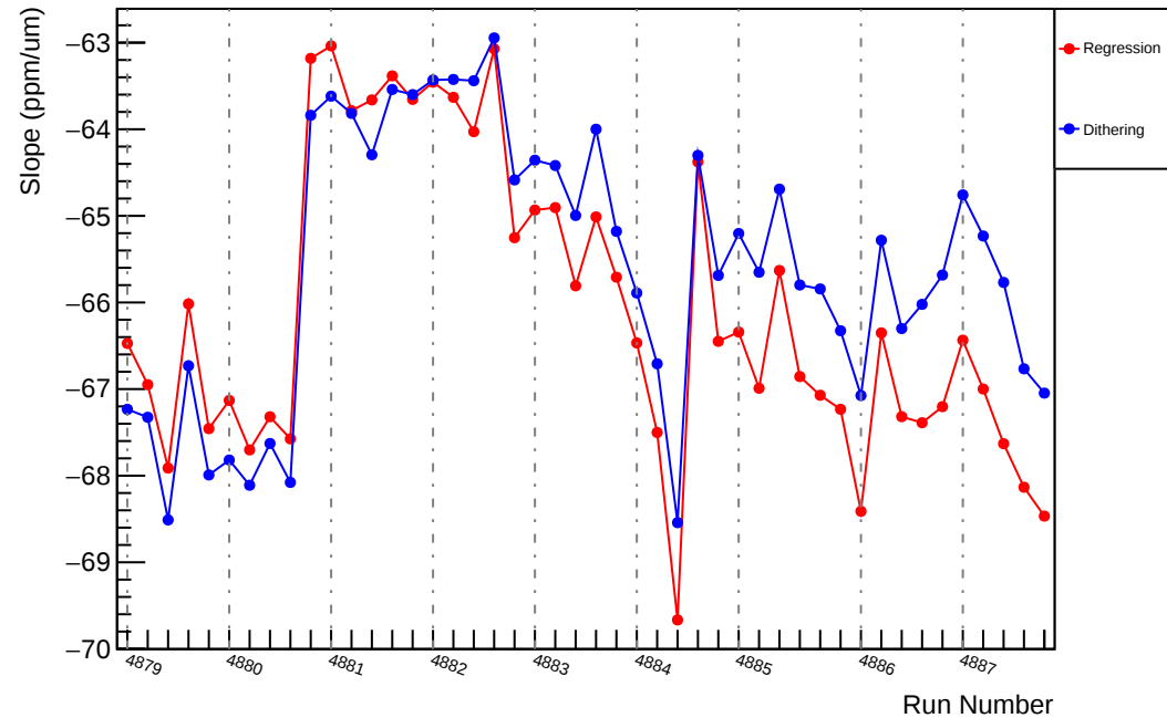
Slug89: Slope : usl_vs_evMon1 (ppm/um)
