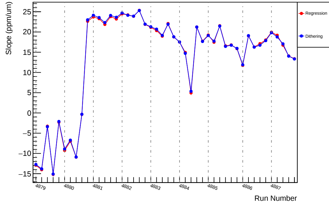
Slug89: Slope : usl_vs_evMon0 (ppm/um)
