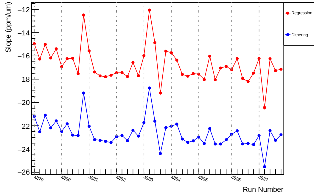
Slug89: Slope : usl_vs_evMon2 (ppm/um)
