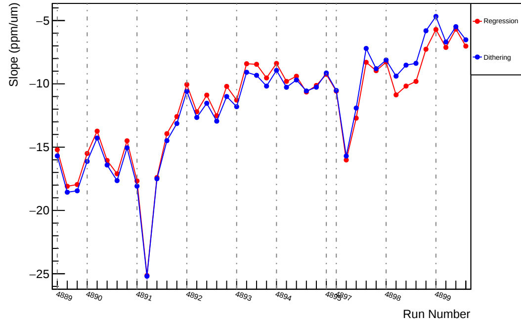
Slug90: Slope : us_avg_vs_evMon0 (ppm/um)
