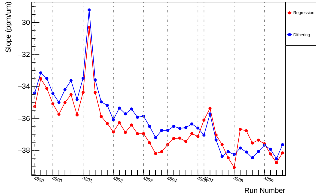
Slug90: Slope : us_avg_vs_evMon1 (ppm/um)
