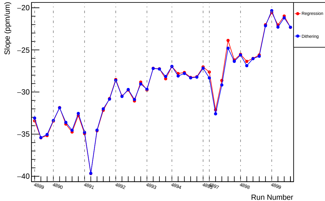
Slug90: Slope : us_dd_vs_evMon1 (ppm/um)
