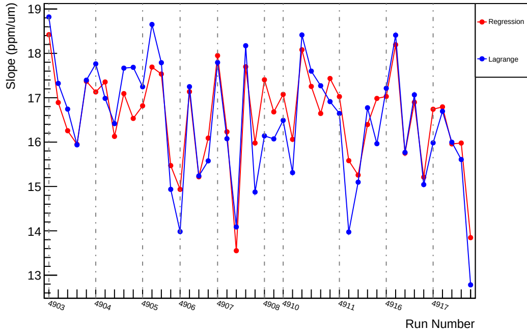
Slug91: Slope : us_avg_vs_evMon6 (ppm/um)
