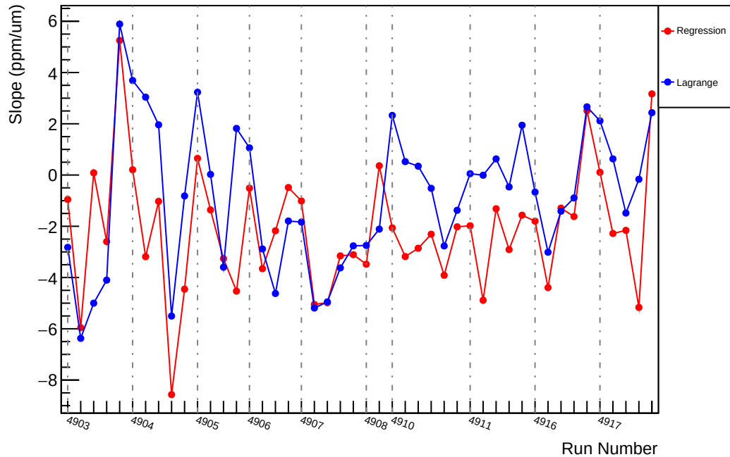
Slug91: Slope : us_avg_vs_evMon8 (ppm/um)
