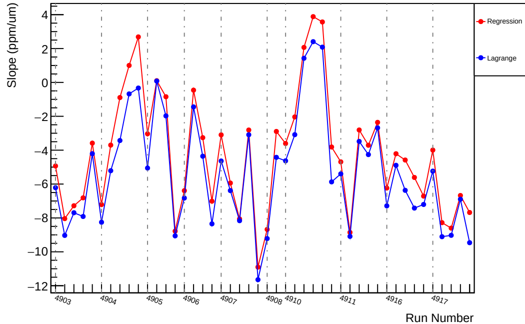
Slug91: Slope : us_avg_vs_evMon7 (ppm/um)
