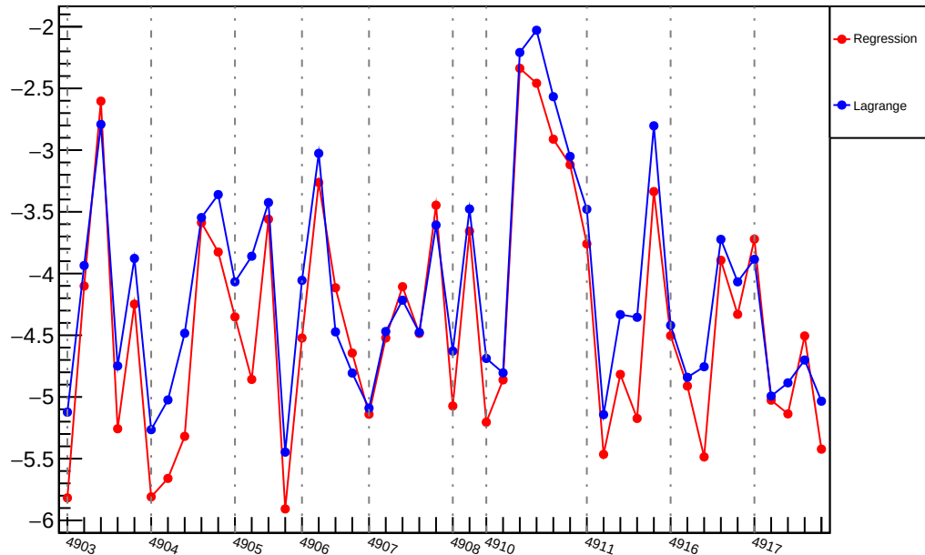
Slug91: Slope : us_dd_vs_evMon5 (ppm/um)
