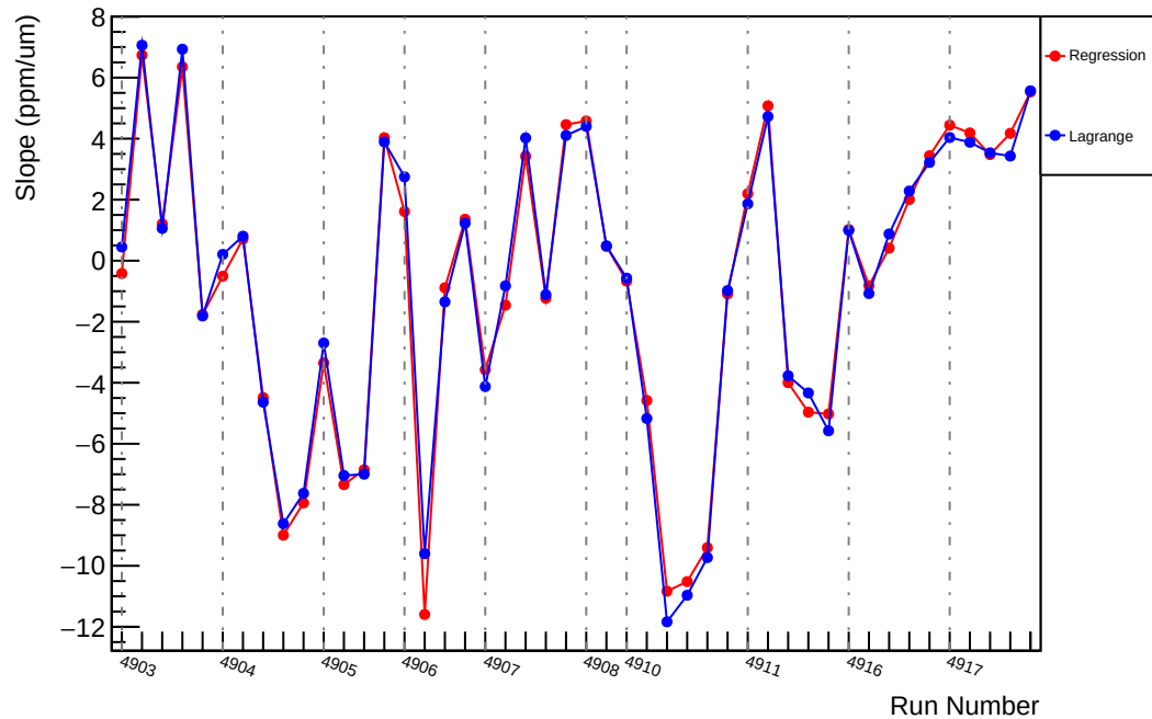
Slug91: Slope : us_dd_vs_evMon6 (ppm/um)
