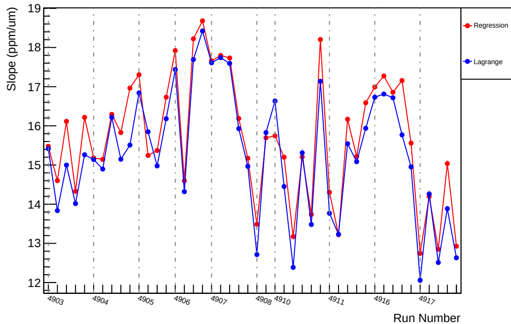
Slug91: Slope : us_dd_vs_evMon7 (ppm/um)
