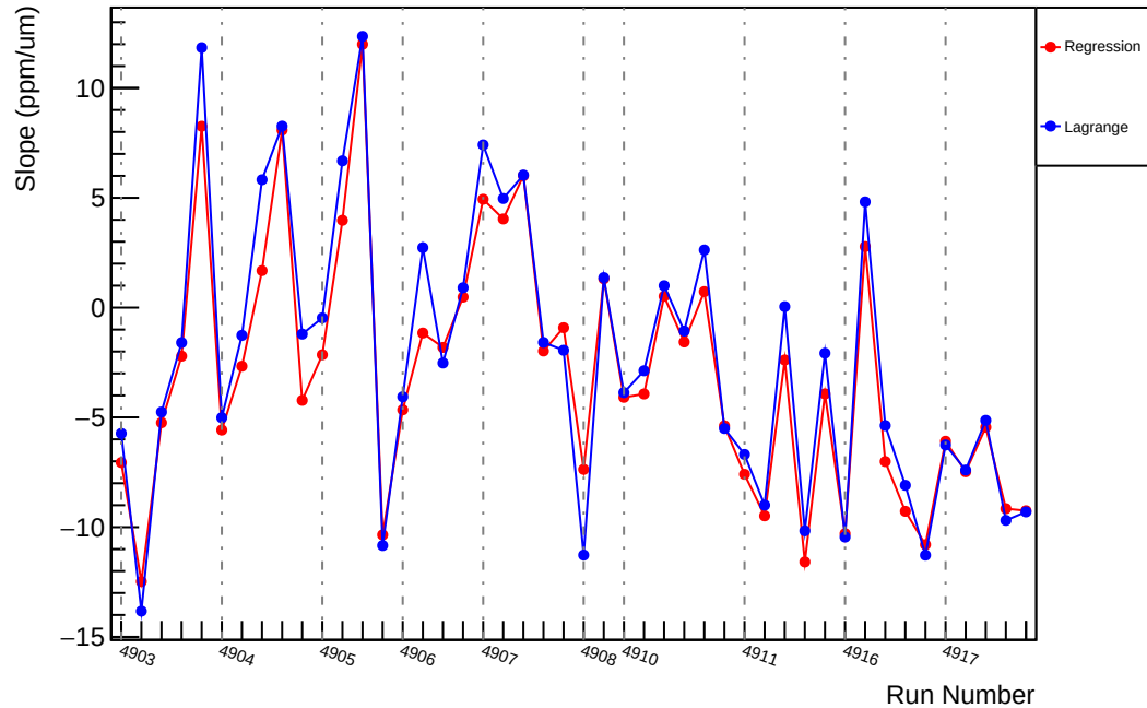
Slug91: Slope : us_dd_vs_evMon9 (ppm/um)
