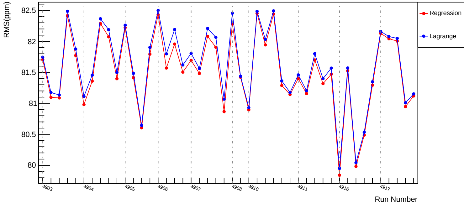
Slug91: Corrected RMS (ppm): asym_us_dd
