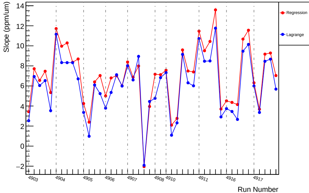
Slug91: Slope : us_dd_vs_evMon10 (ppm/um)
