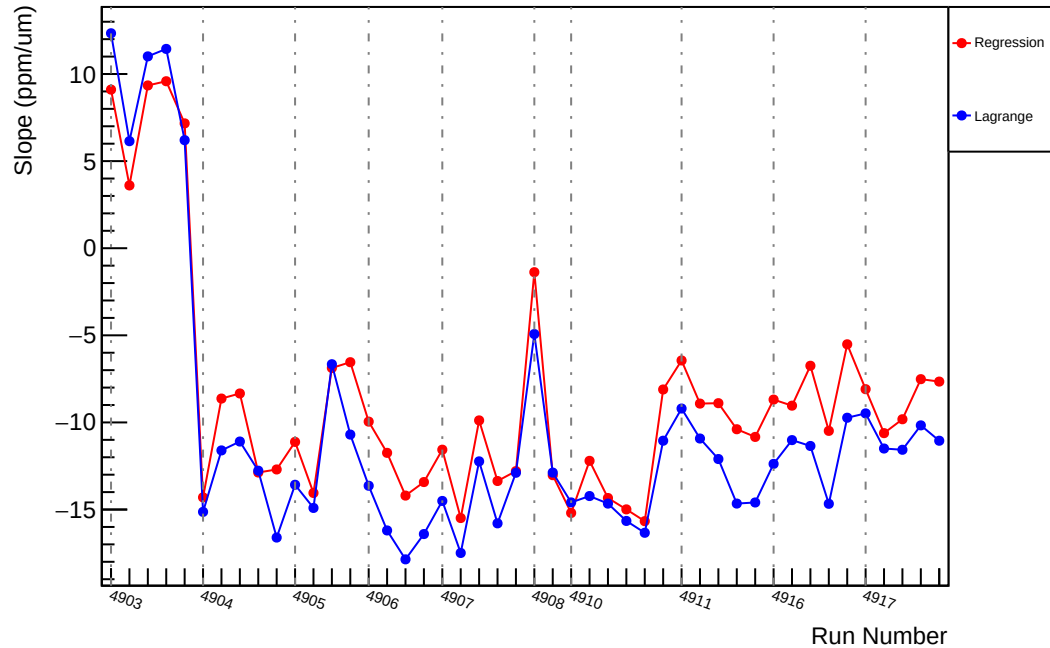
Slug91: Slope : us_dd_vs_evMon8 (ppm/um)
