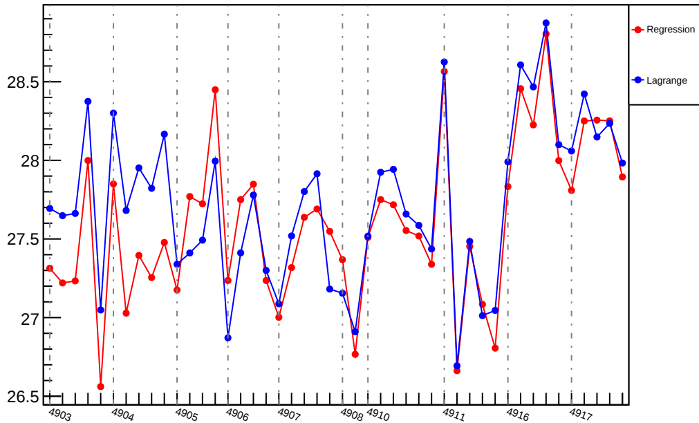
Slug91: Slope : usr_vs_evMon0 (ppm/um)
