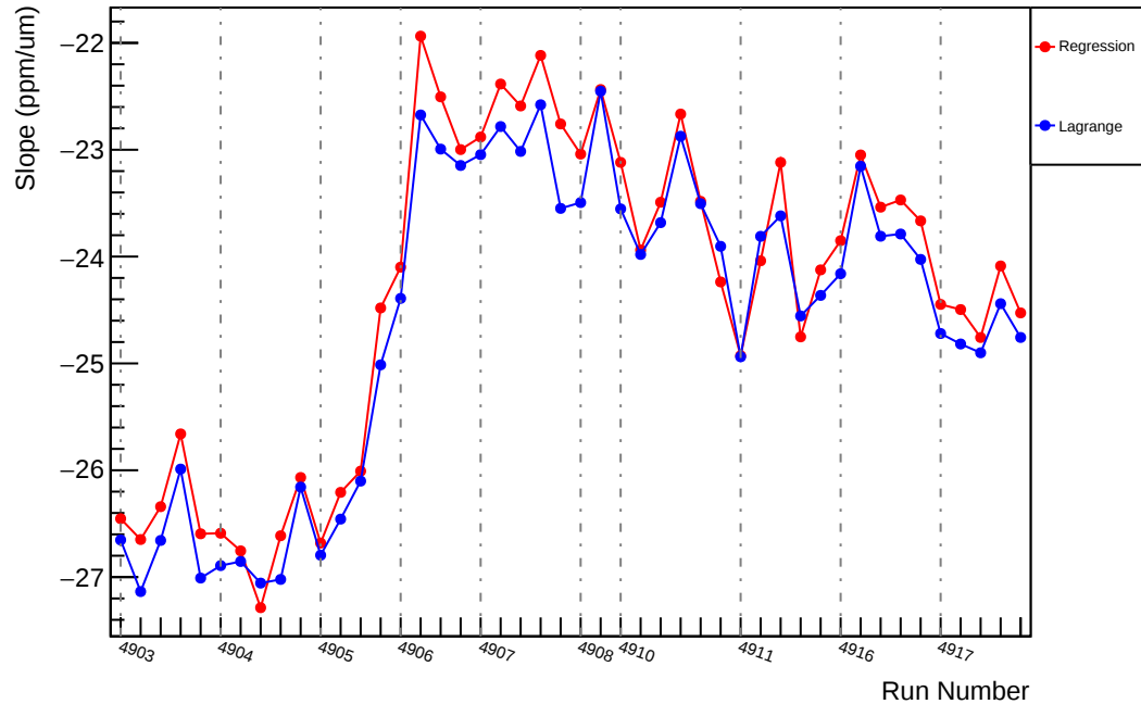
Slug91: Slope : usr_vs_evMon1 (ppm/um)
