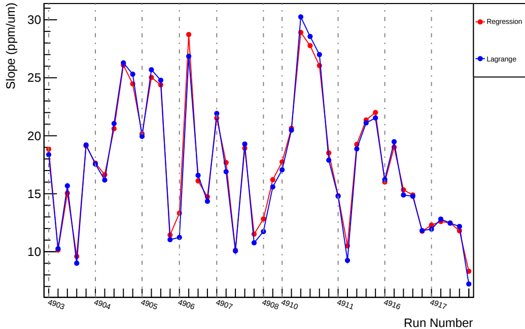
Slug91: Slope : usr_vs_evMon6 (ppm/um)
