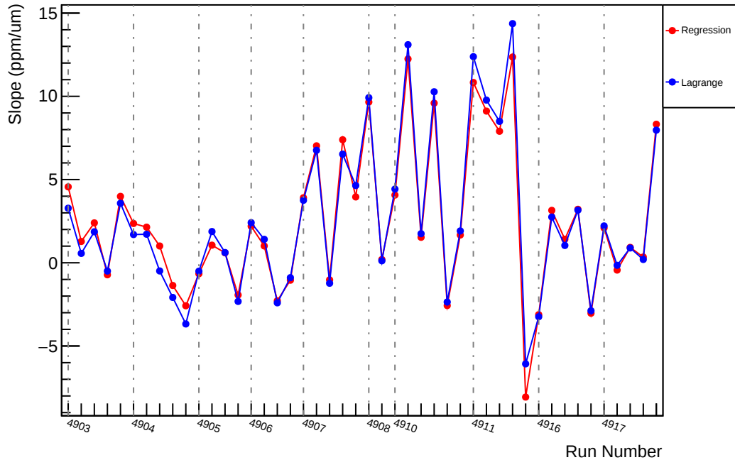
Slug91: Slope : usr_vs_evMon11 (ppm/um)
