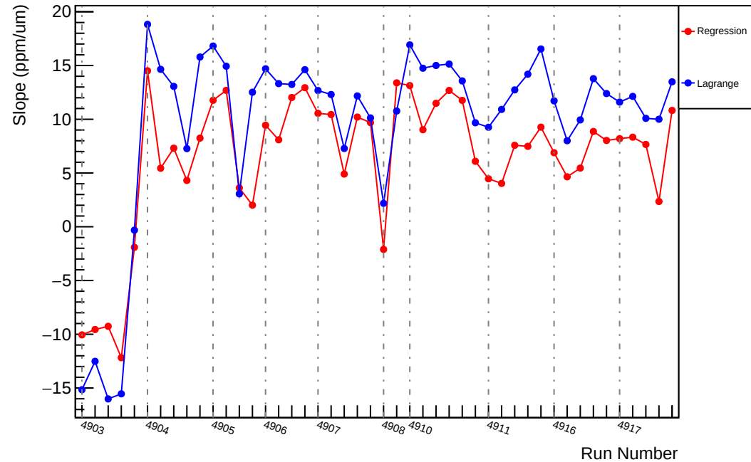
Slug91: Slope : usr_vs_evMon8 (ppm/um)
