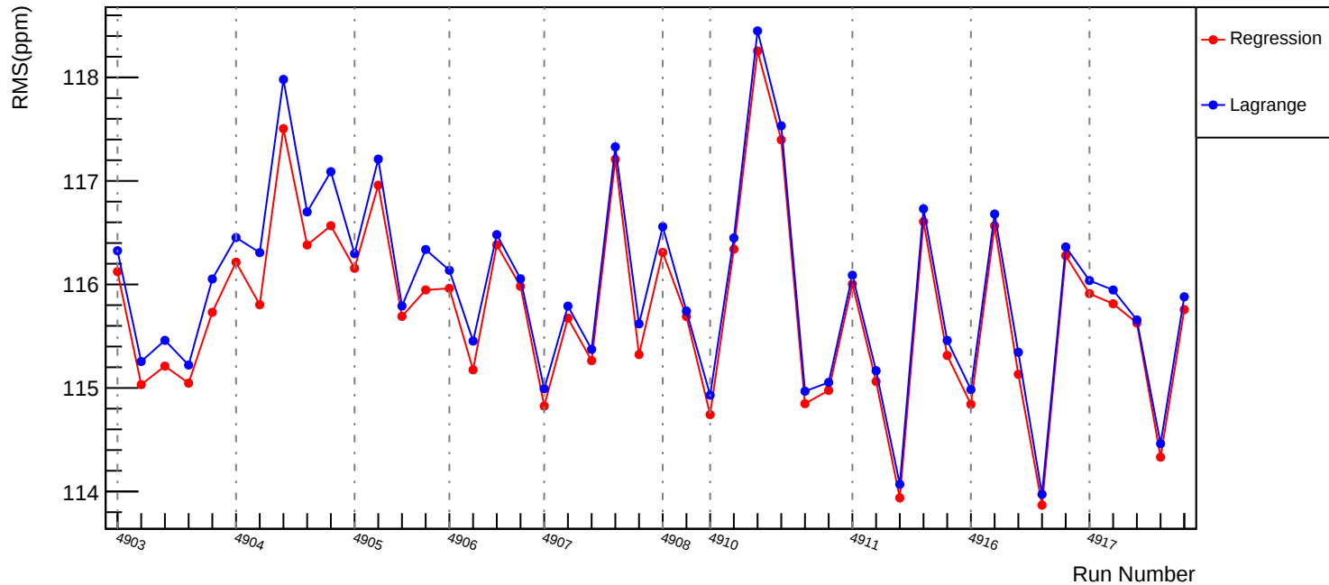
Slug91: Corrected RMS (ppm): asym_usr
