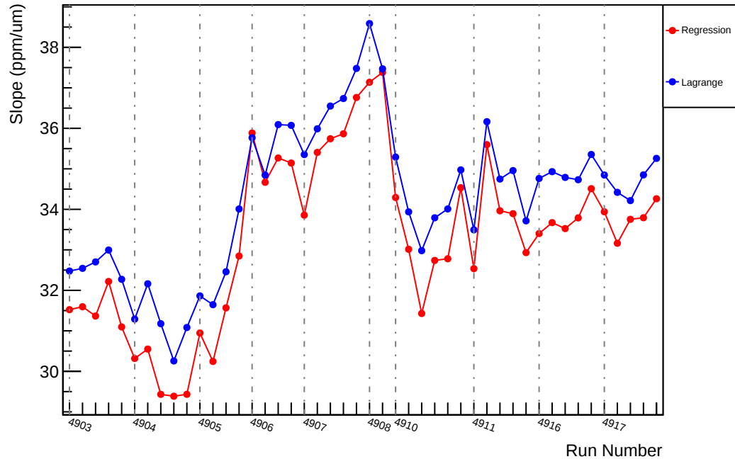
Slug91: Slope : usr_vs_evMon2 (ppm/um)
