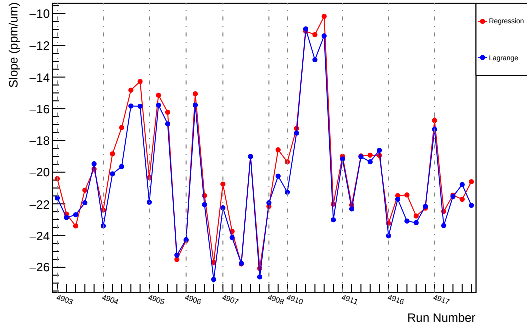
Slug91: Slope : usr_vs_evMon7 (ppm/um)
