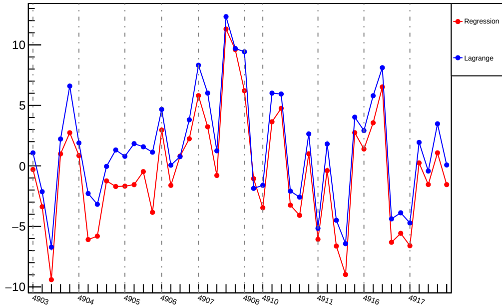
Slug91: Slope : usr_vs_evMon10 (ppm/um)
