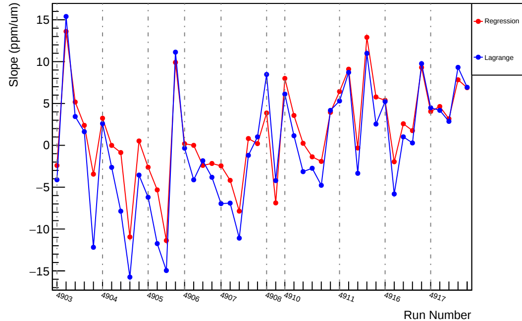
Slug91: Slope : usr_vs_evMon9 (ppm/um)
