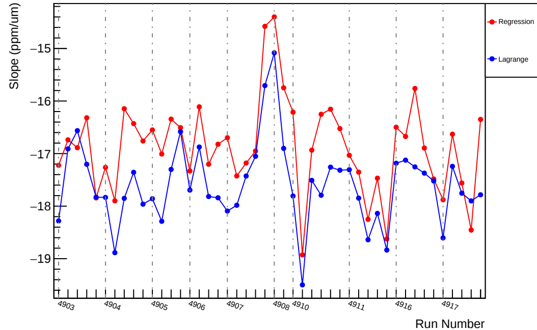
Slug91: Slope : usr_vs_evMon4 (ppm/um)
