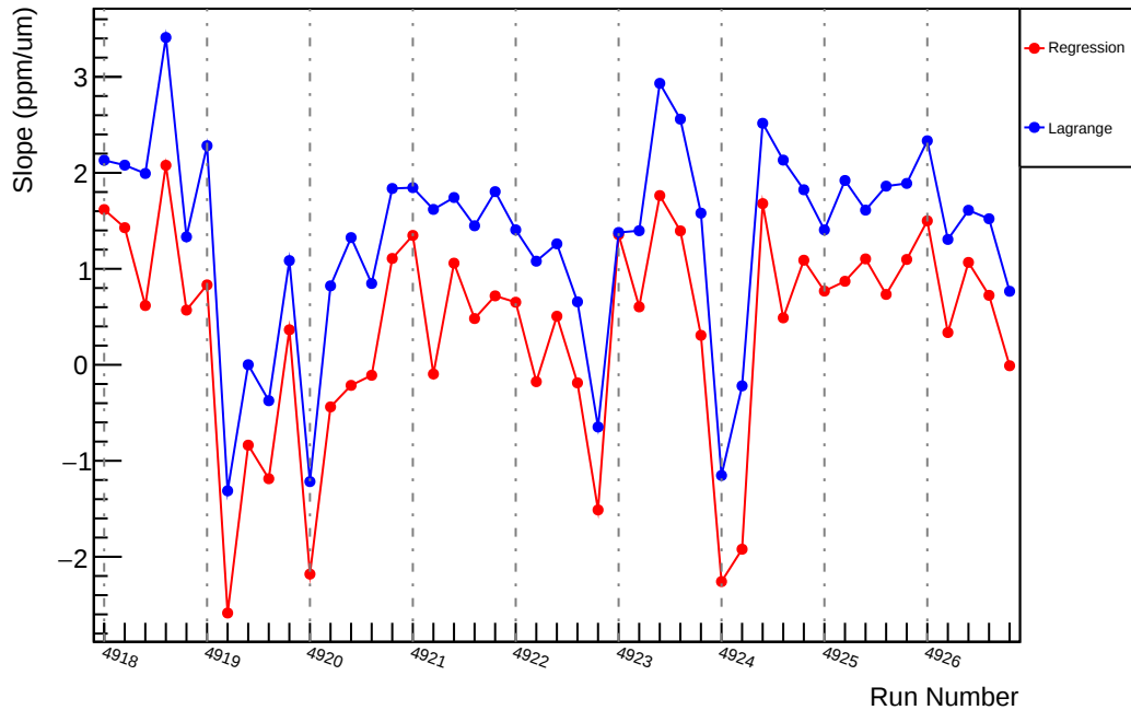
Slug92: Slope : us_dd_vs_evMon2 (ppm/um)
