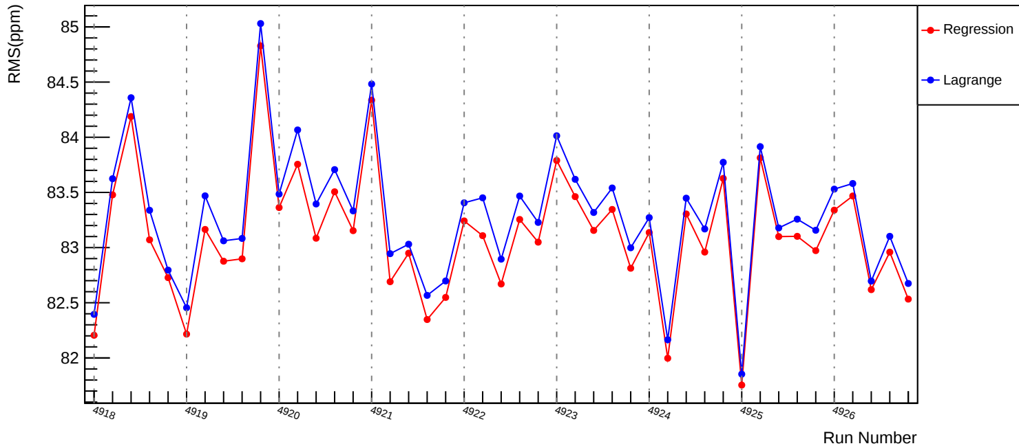
Slug92: Corrected RMS (ppm): asym_us_dd
