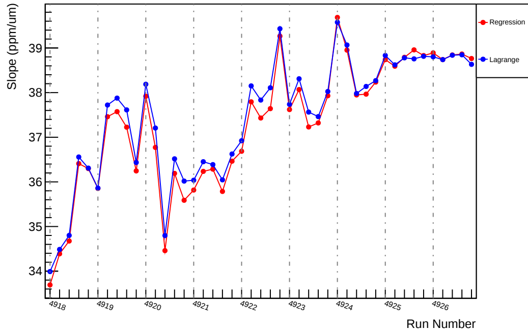
Slug92: Slope : us_dd_vs_evMon0 (ppm/um)
