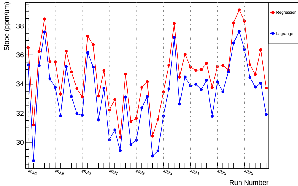
Slug92: Slope : us_dd_vs_evMon4 (ppm/um)
