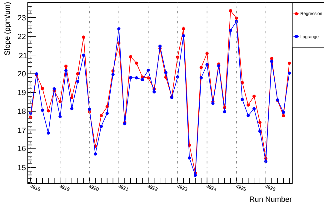
Slug92: Slope : usl_vs_evMon6 (ppm/um)
