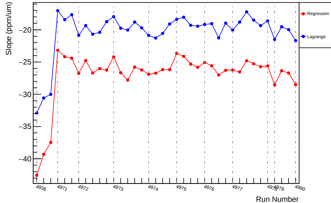
Slug94: Slope : us_avg_vs_evMon3 (ppm/um)
