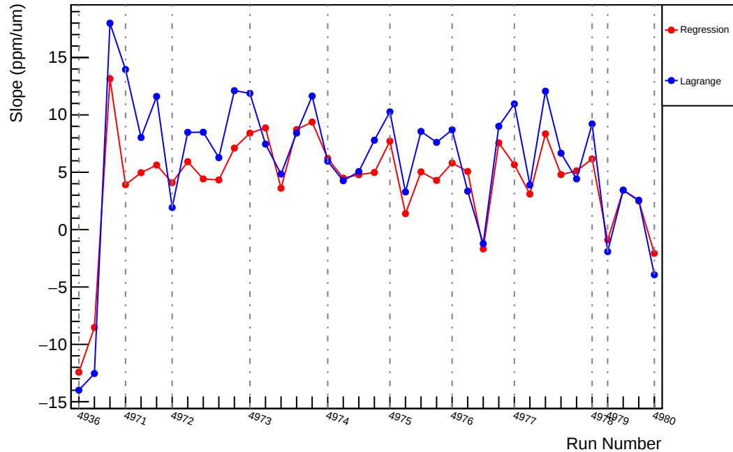
Slug94: Slope : us_avg_vs_evMon5 (ppm/um)
