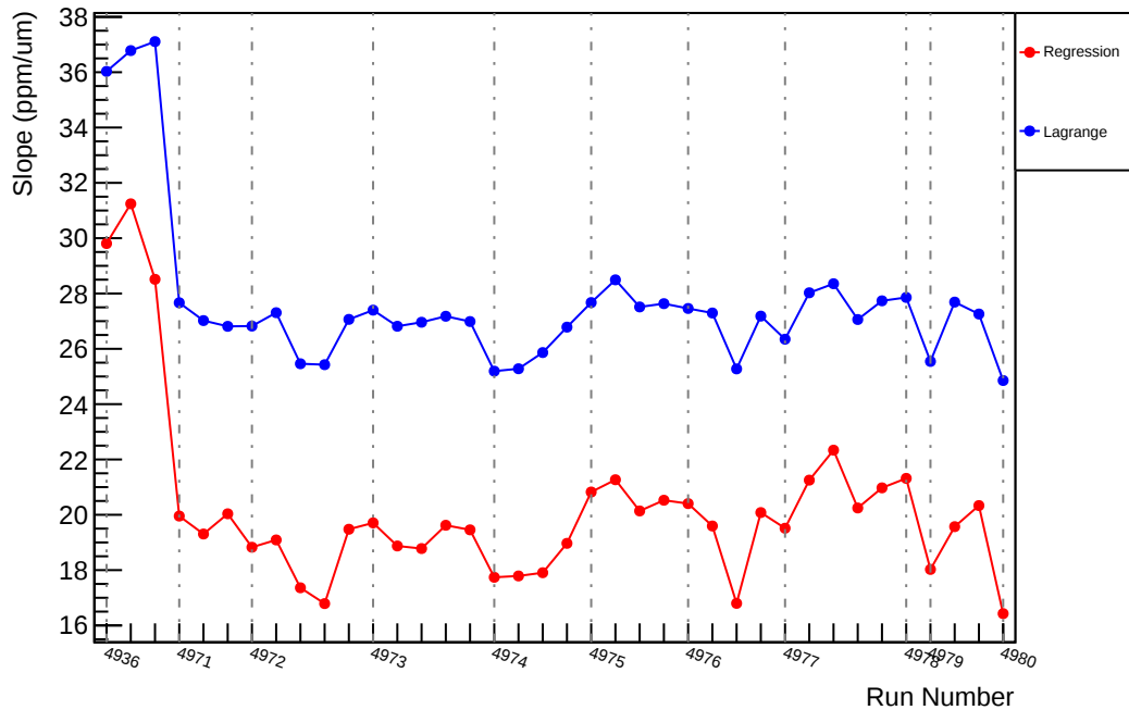
Slug94: Slope : us_avg_vs_evMon2 (ppm/um)
