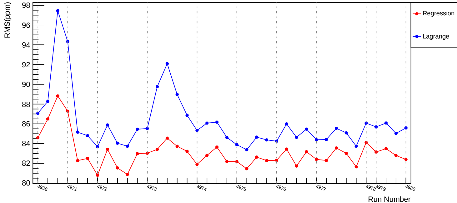
Slug94: Corrected RMS (ppm): asym_us_avg
