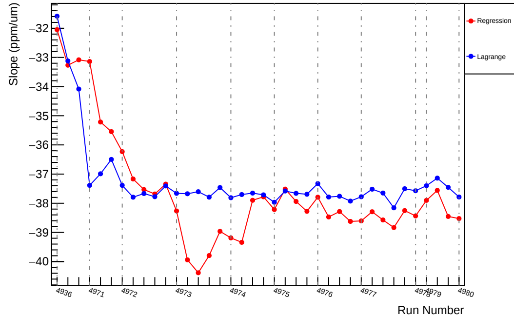
Slug94: Slope : us_avg_vs_evMon1 (ppm/um)
