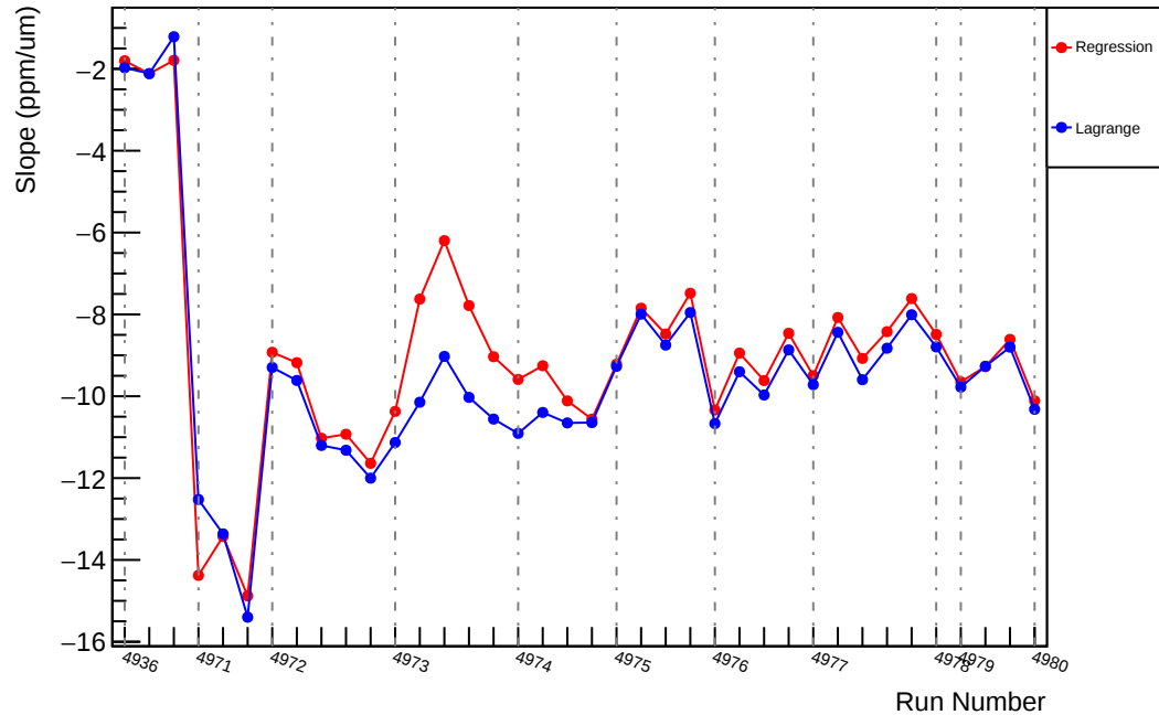
Slug94: Slope : us_avg_vs_evMon0 (ppm/um)
