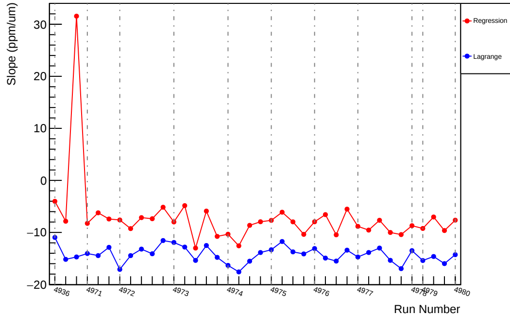
Slug94: Slope : us_avg_vs_evMon4 (ppm/um)
