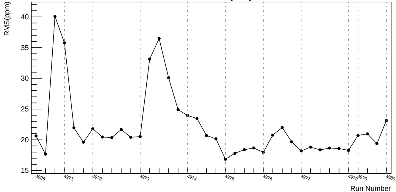
Slug94: asym_us_avg: \sqrt{\sigma_{\text{lagr}}^2 - \sigma_{\text{reg}}^2} (ppm)
