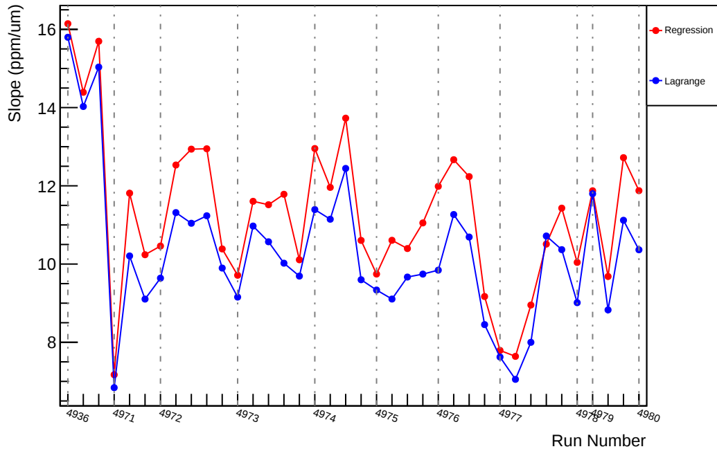
Slug94: Slope : us_dd_vs_evMon7 (ppm/um)
