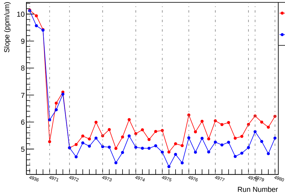
Slug94: Slope : us_dd_vs_evMon1 (ppm/um)
