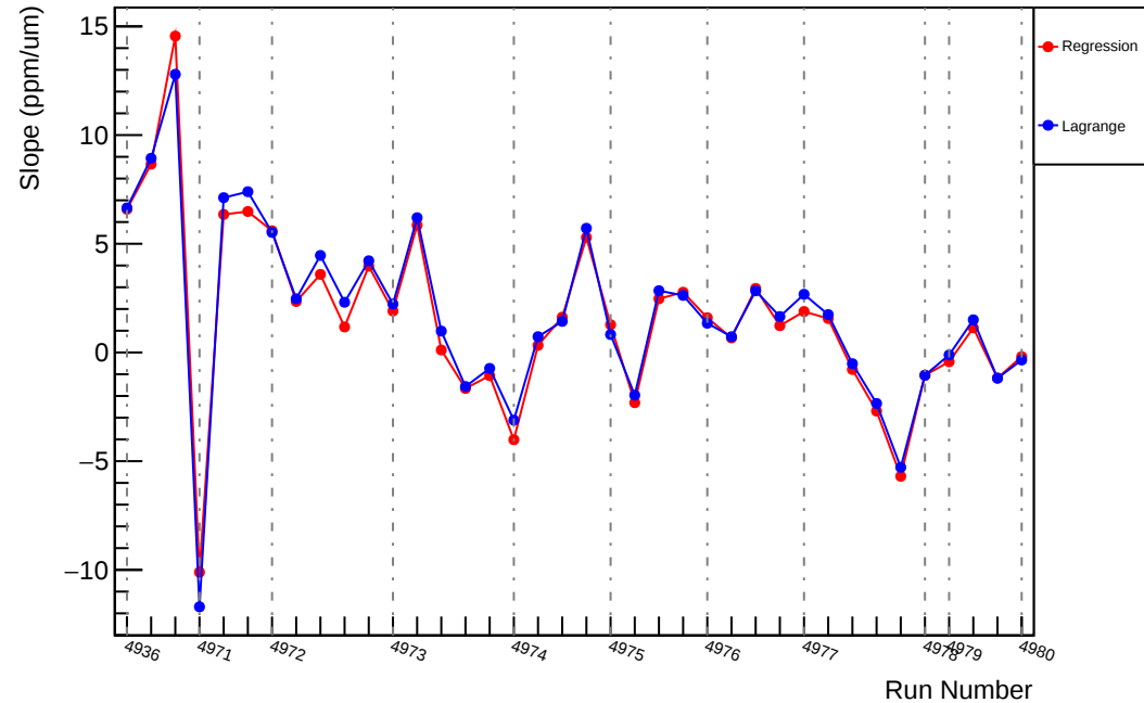
Slug94: Slope : us_dd_vs_evMon11 (ppm/um)
