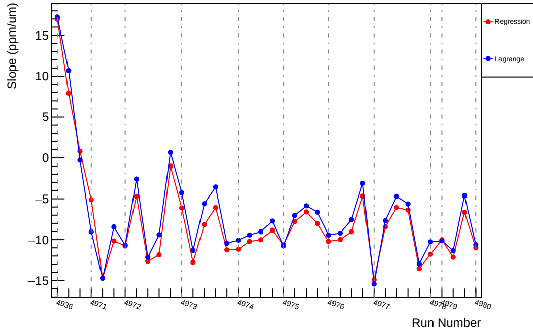
Slug94: Slope : us_dd_vs_evMon8 (ppm/um)
