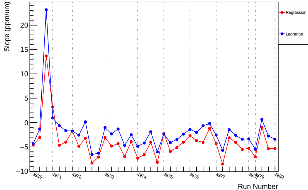
Slug94: Slope : us_dd_vs_evMon10 (ppm/um)
