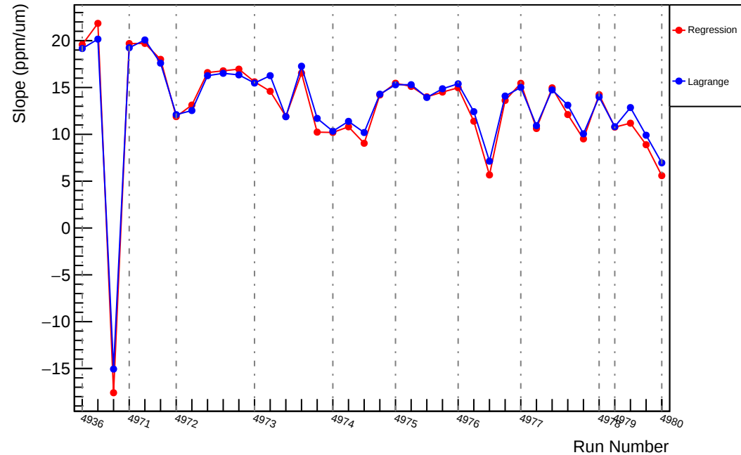
Slug94: Slope : usl_vs_evMon6 (ppm/um)
