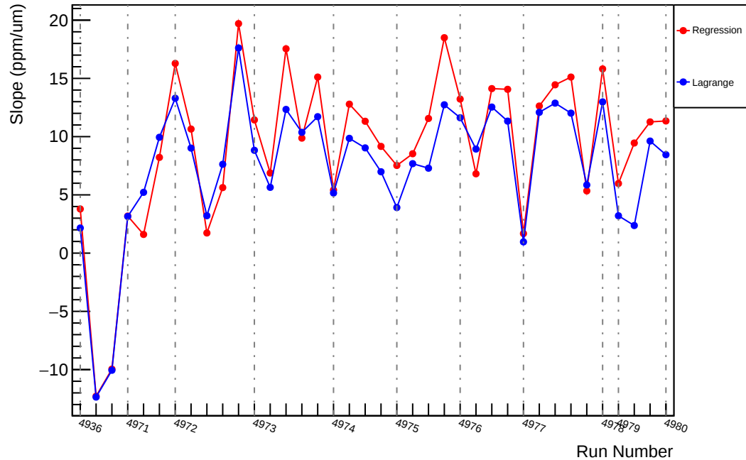
Slug94: Slope : usl_vs_evMon9 (ppm/um)
