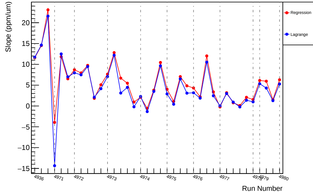
Slug94: Slope : usl_vs_evMon11 (ppm/um)
