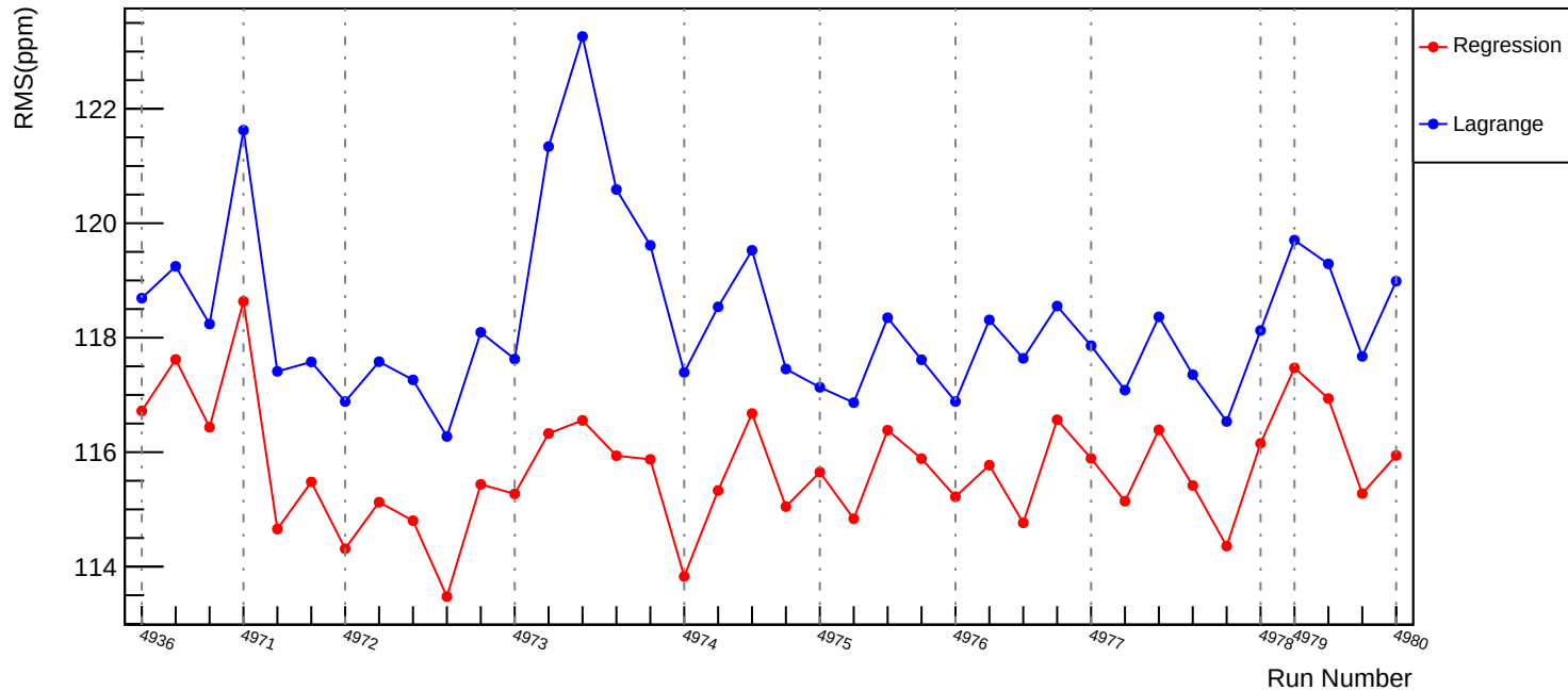
Slug94: Corrected RMS (ppm): asym_usr
