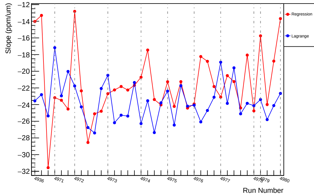
Slug94: Slope : usr_vs_evMon5 (ppm/um)
