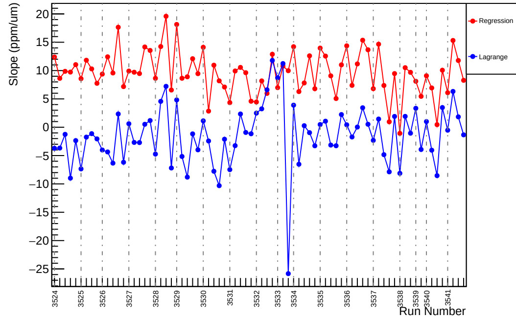
Slug9: Slope : usl_vs_evMon9 (ppm/um)
