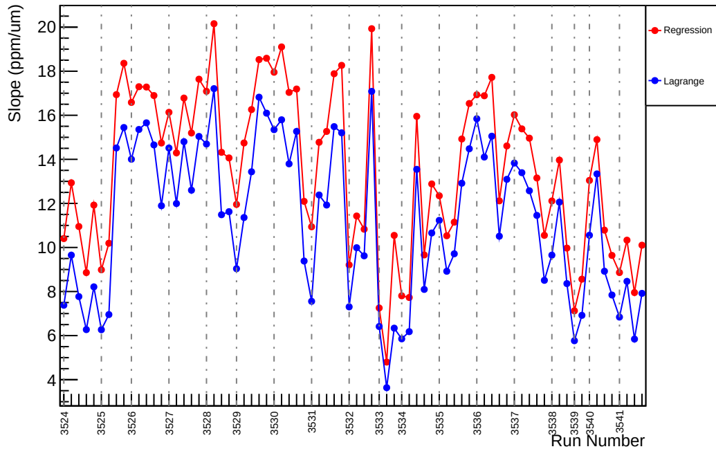
Slug9: Slope : usl_vs_evMon5 (ppm/um)
