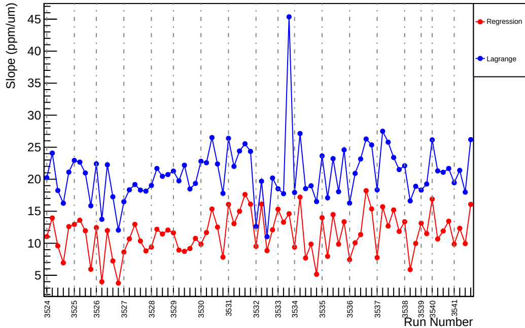
Slug9: Slope : usl_vs_evMon8 (ppm/um)
