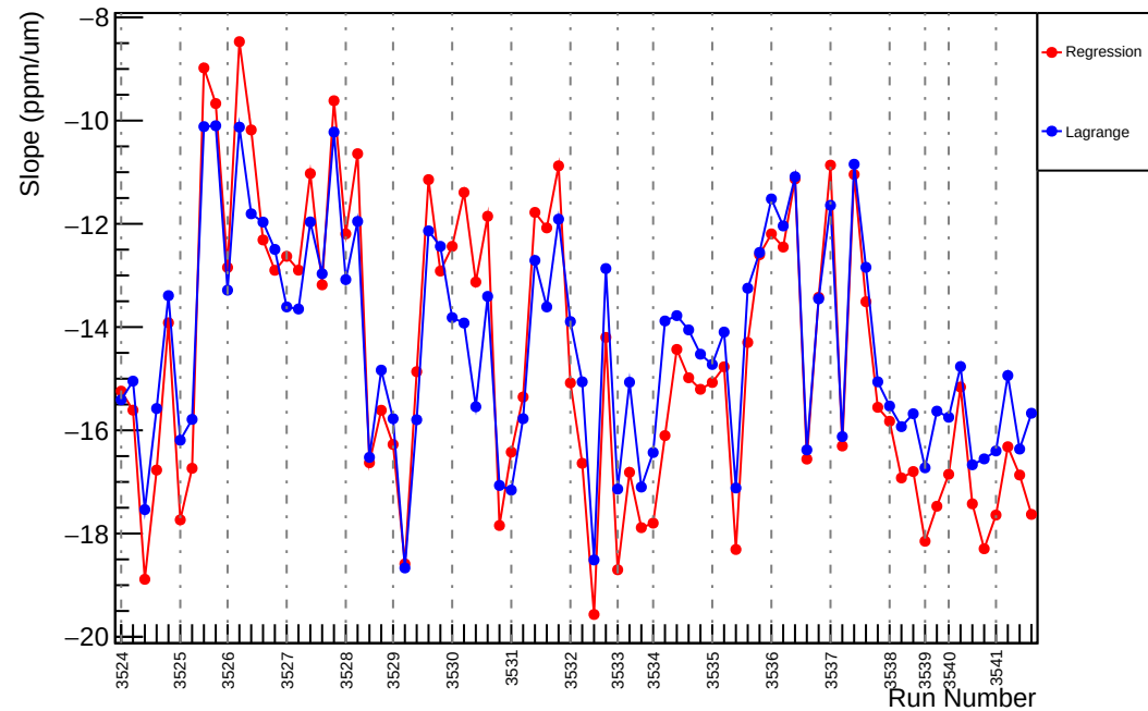
Slug9: Slope : usl_vs_evMon6 (ppm/um)
