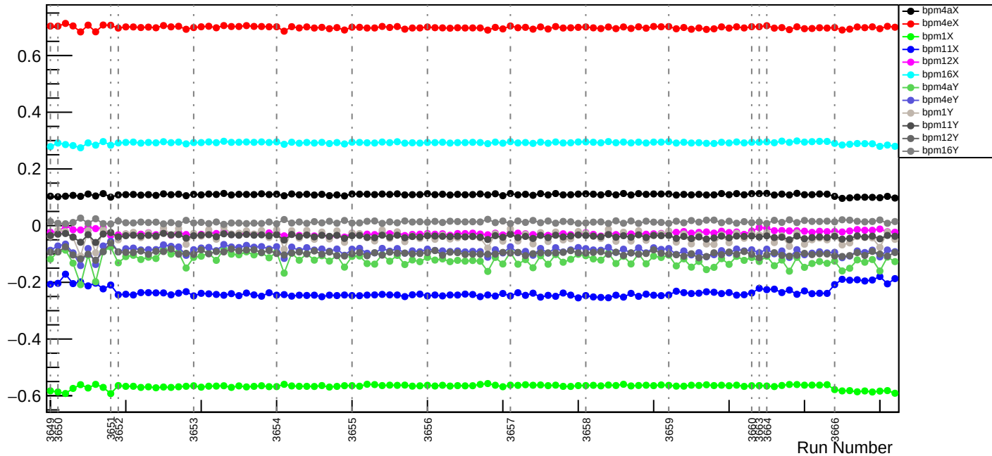
Slug14: EigenVector #0
