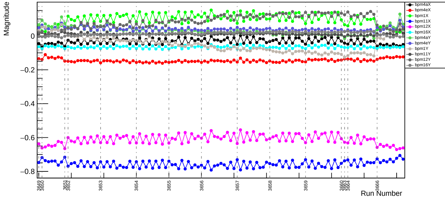
Slug14: EigenVector #2
