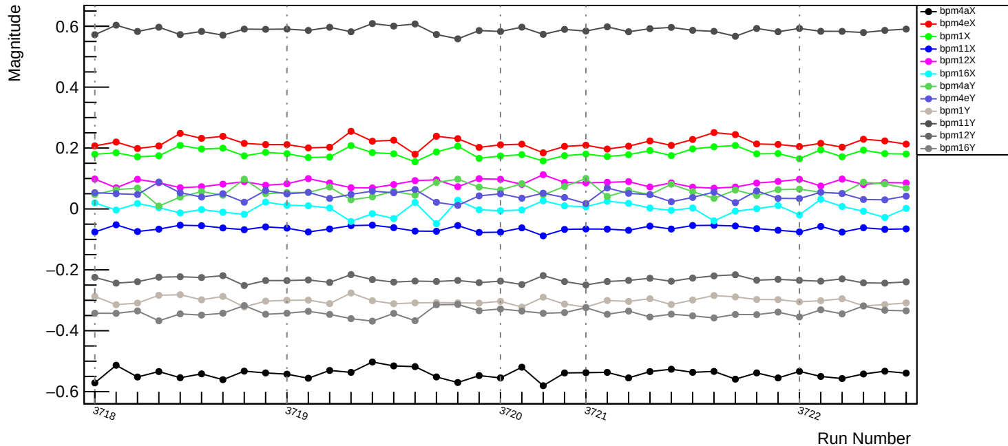
Slug20: EigenVector #9
