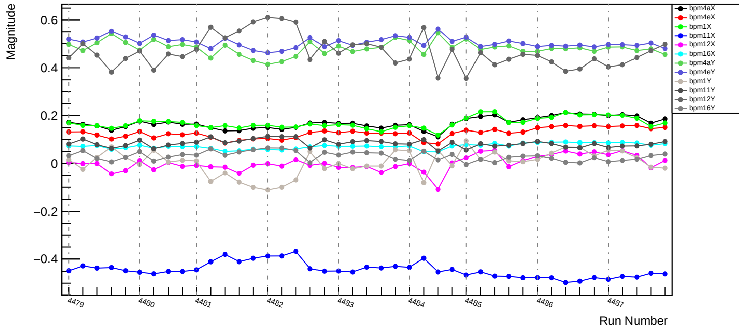
Slug61: EigenVector #1
