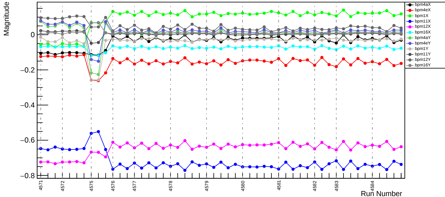
Slug69: EigenVector #2
