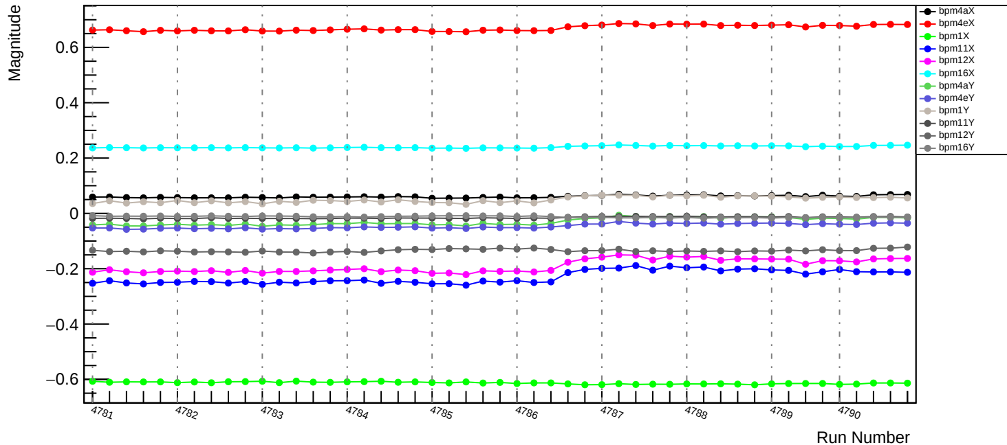
Slug81: EigenVector #0
