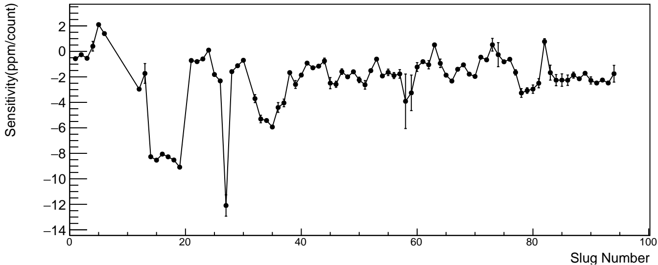
us_avg vs coil 5 Raw sensitivity(ppm/count)
