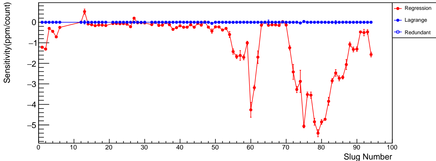
us_avg vs coil 4 Raw sensitivity(ppm/count)
