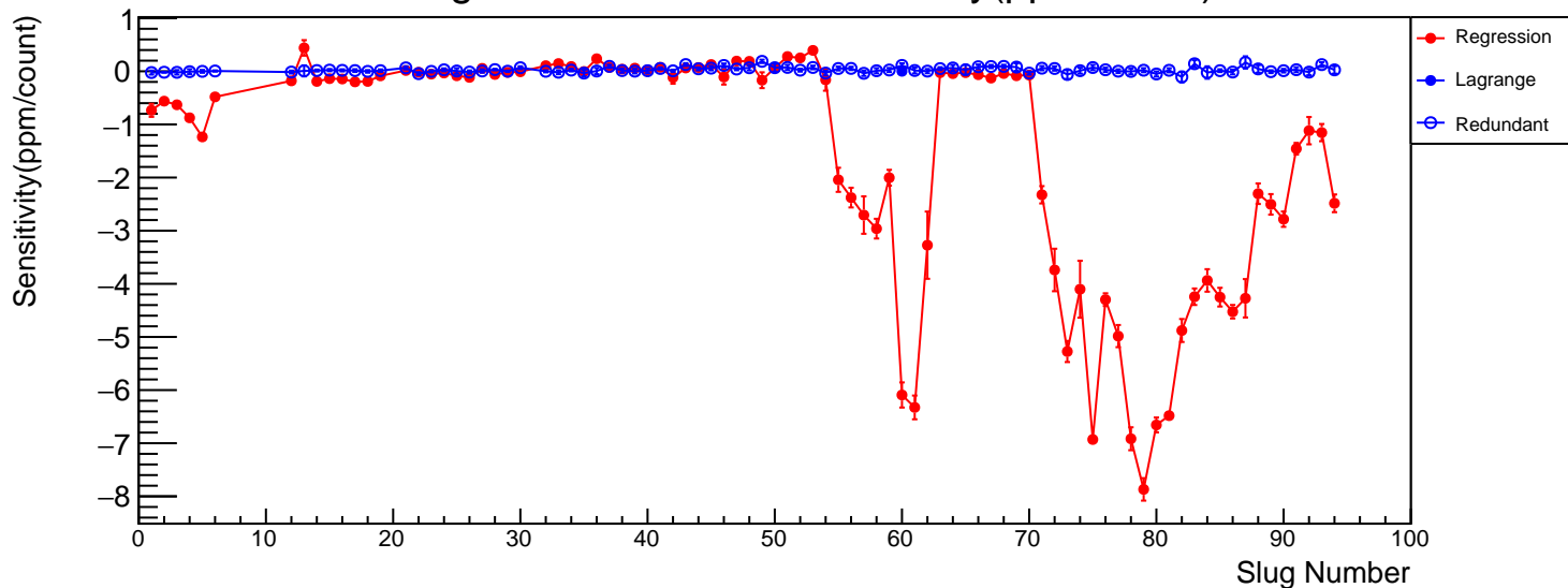
us_avg vs coil 2 Raw sensitivity(ppm/count)
