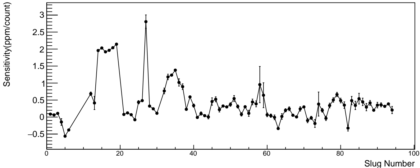
us_avg vs coil 3 Raw sensitivity(ppm/count)
