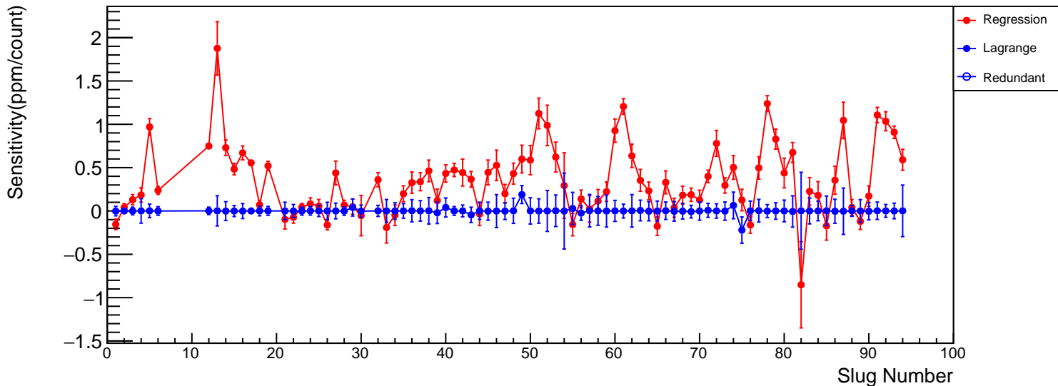
us_avg vs coil 7 Raw sensitivity(ppm/count)
