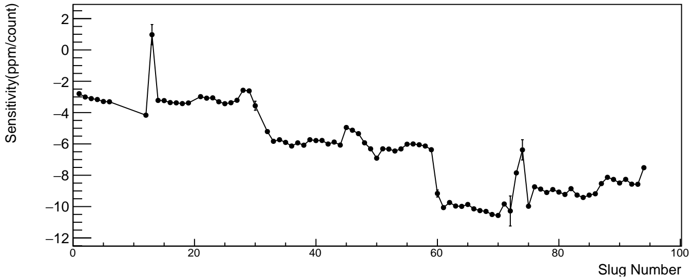
us_avg vs coil 4 Raw sensitivity(ppm/count)
