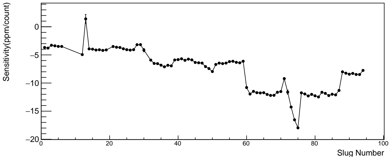
us_avg vs coil 2 Raw sensitivity(ppm/count)
