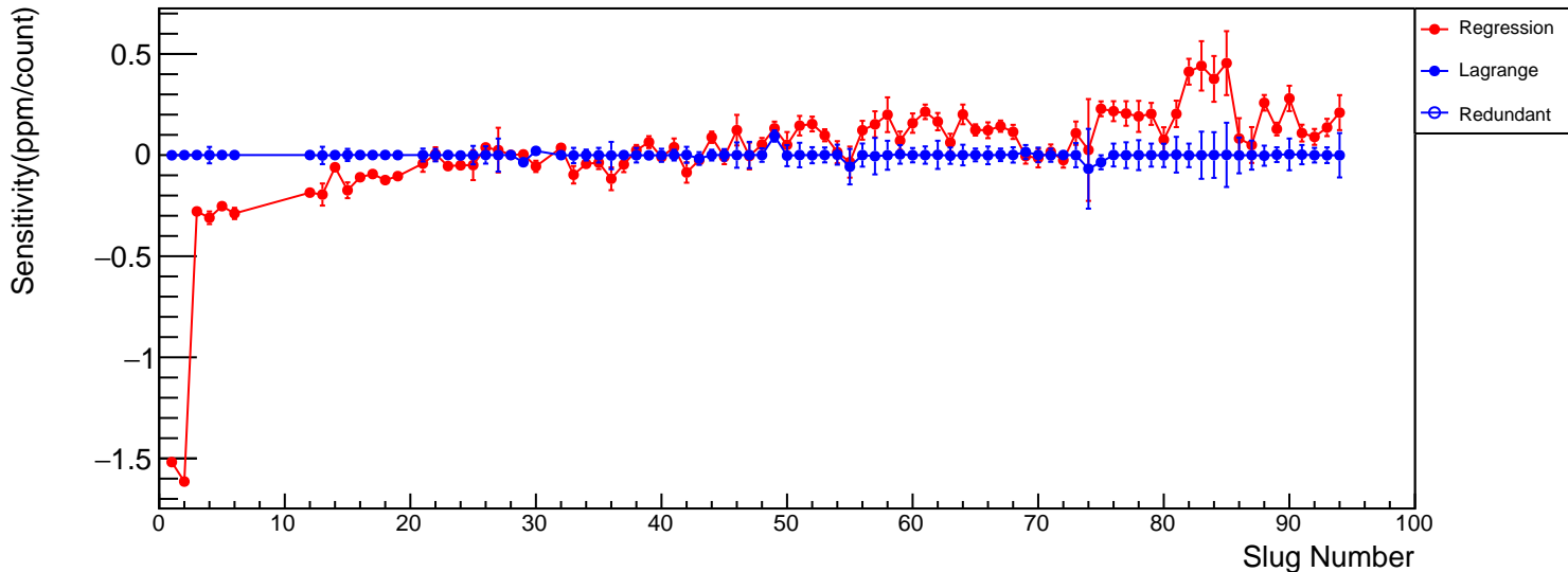
us_avg vs coil 3 Raw sensitivity(ppm/count)
