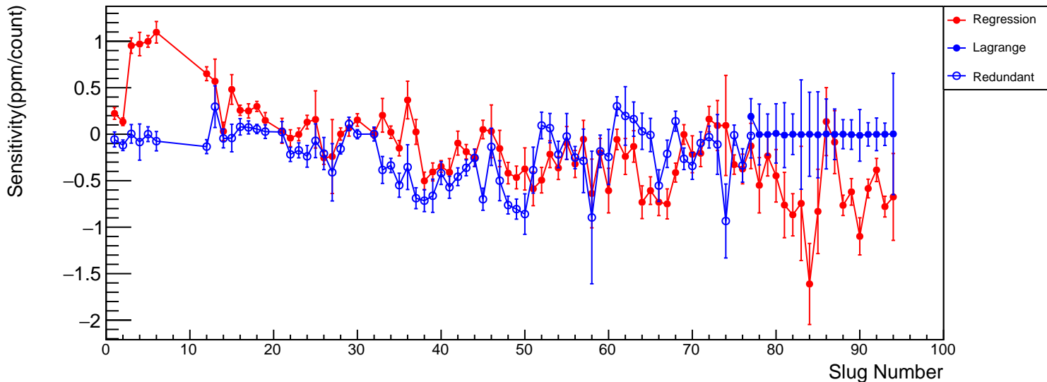
us_avg vs coil 5 Raw sensitivity(ppm/count)
