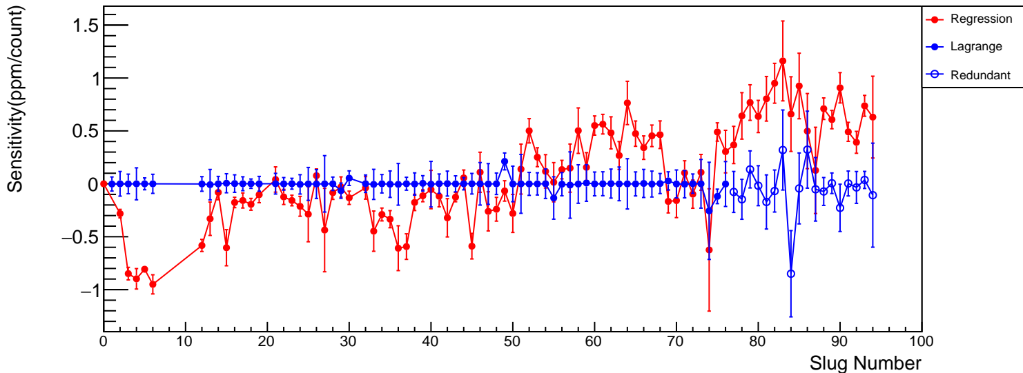
us_avg vs coil 1 Raw sensitivity(ppm/count)
