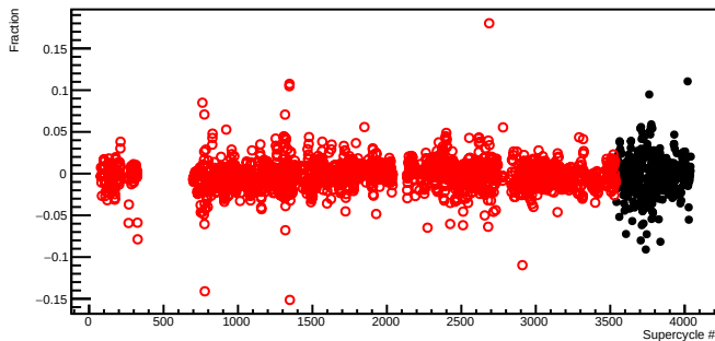
usr_coil5 Fractional Residual
