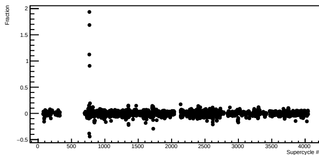
usr_coil4 Fractional Residual
