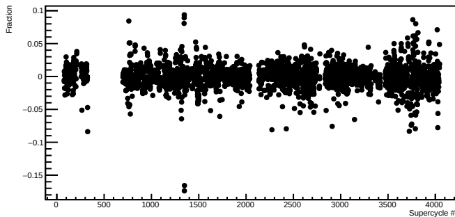
usr_coil3 Fractional Residual
