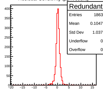
Residual Sensitivity (ppm/count)
