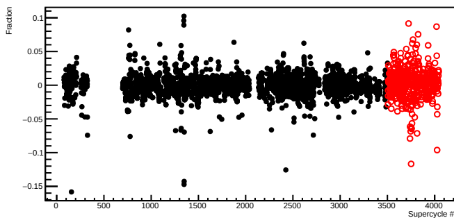
usr_coil1 Fractional Residual
