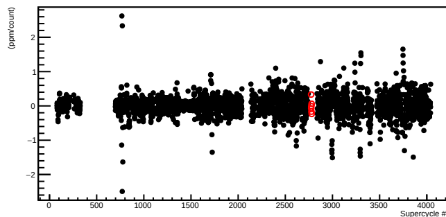
usr_coil6 Residual (ppm/count)
