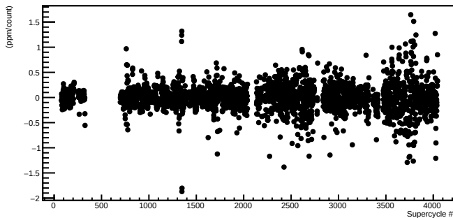
usr_coil3 Residual (ppm/count)
