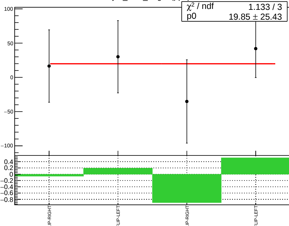
asym_bcm_target (ppb)
