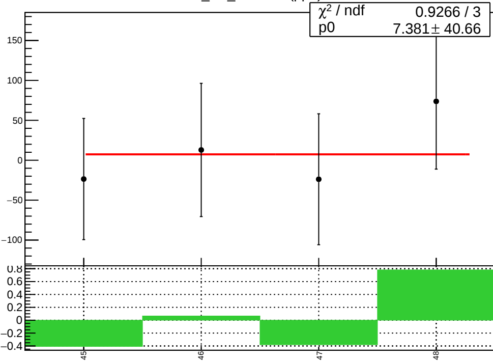
corr_usl_evMon1 (ppb)
