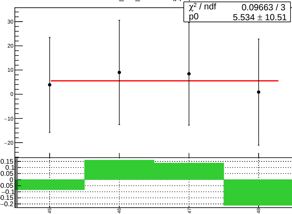
corr_usr_evMon3 (ppb)
