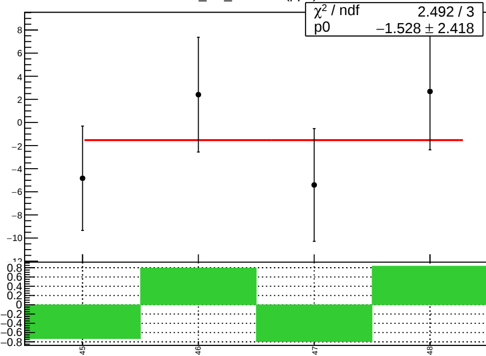
corr_usl_evMon5 (ppb)
