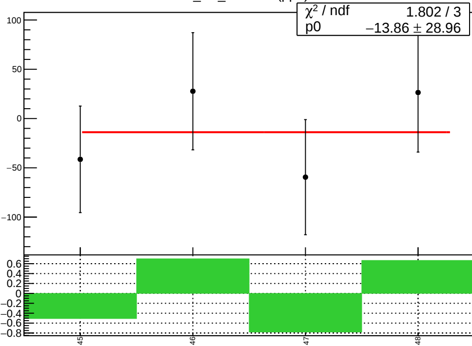
corr_usl_evMon4 (ppb)
