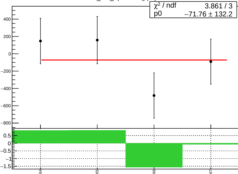
corr_usr_bpm4eX (ppb)
