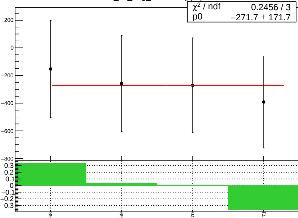
corr_us_avg_evMon2 (ppb)
