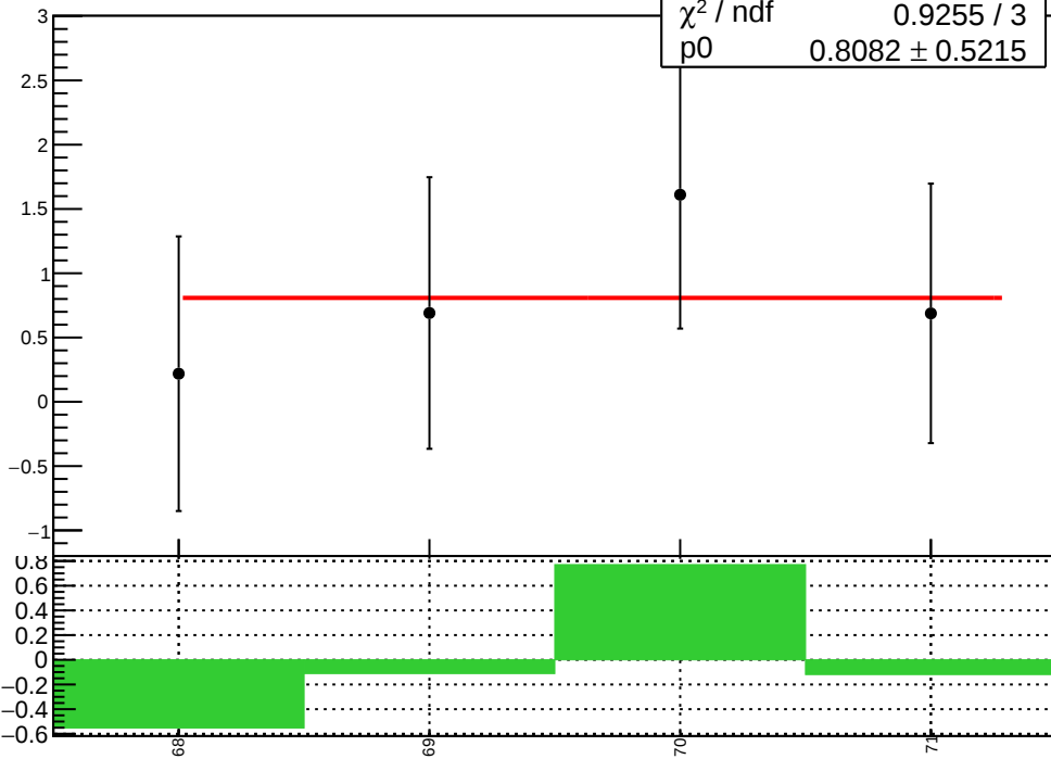
diff_evMon7 (nm)
