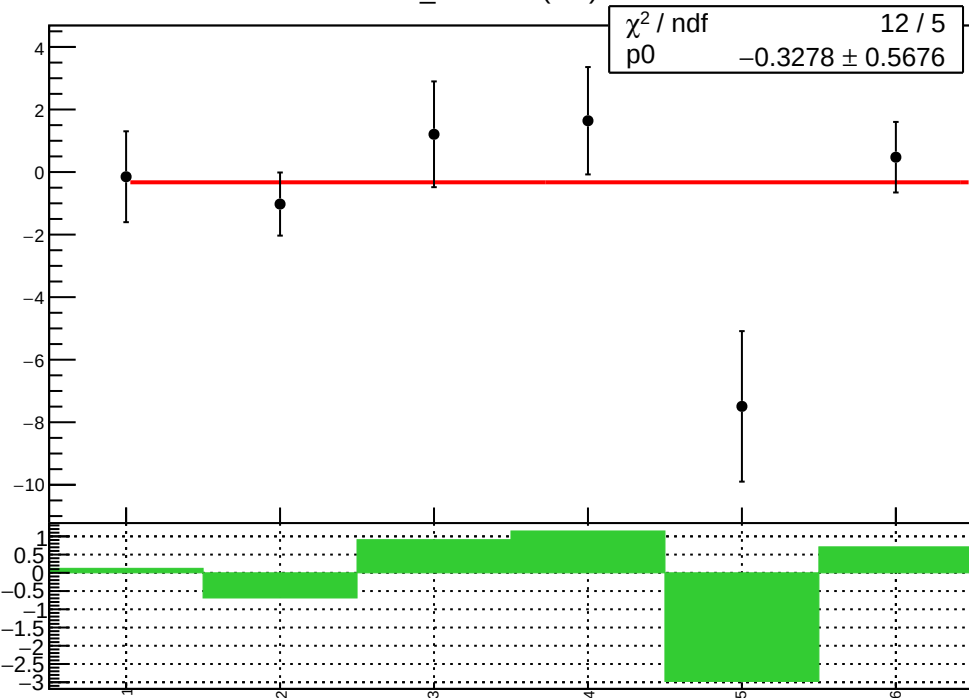
diff_evMon6 (nm)
