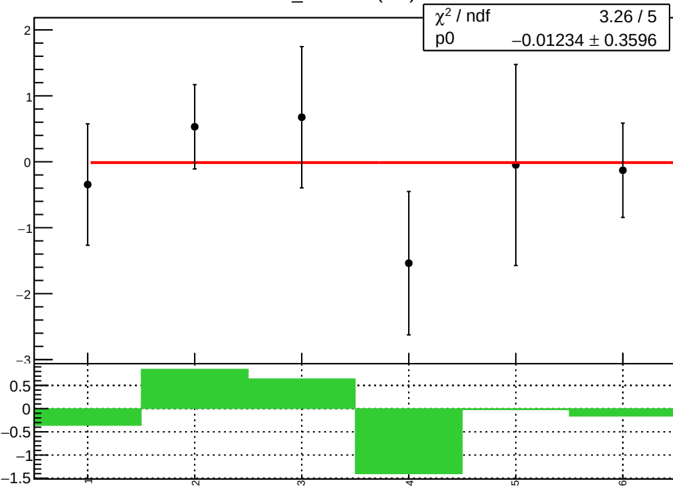
diff_evMon9 (nm)
