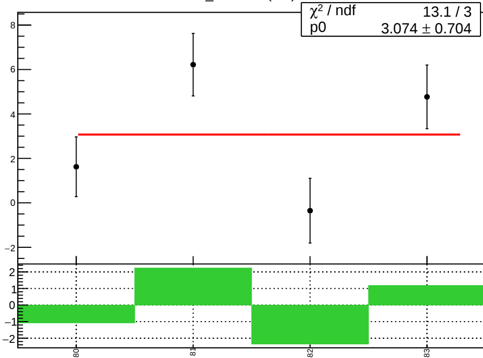
diff_evMon6 (nm)
