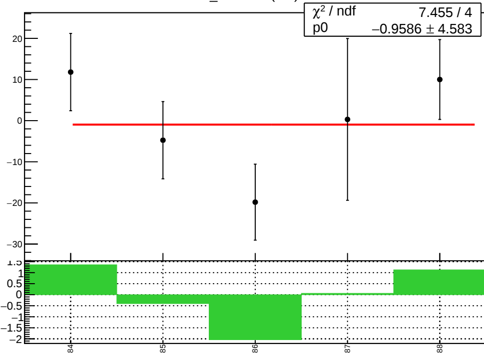
diff_evMon2 (nm)
