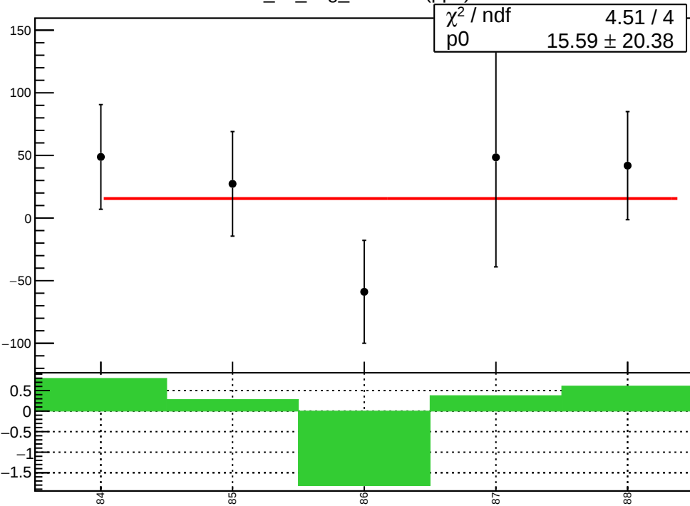
corr_us_avg_evMon3 (ppb)
