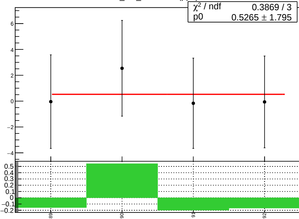
corr_usr_evMon11 (ppb)
