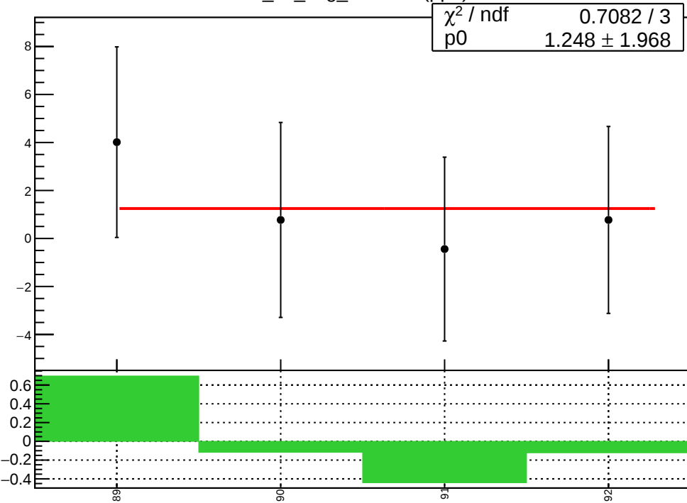
corr_us_avg_evMon9 (ppb)
