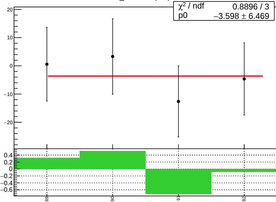
diff_evMon1 (nm)
