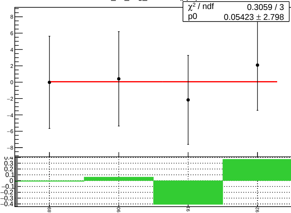
corr_us_avg_evMon8 (ppb)
