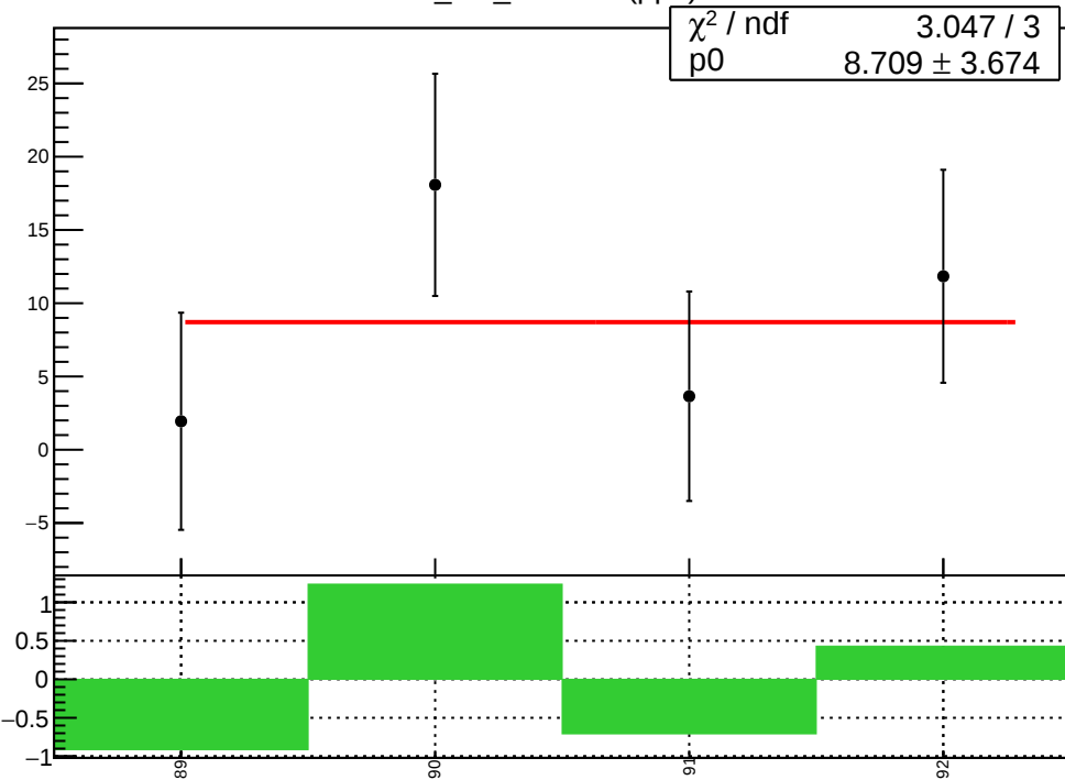
corr_usr_evMon5 (ppb)
