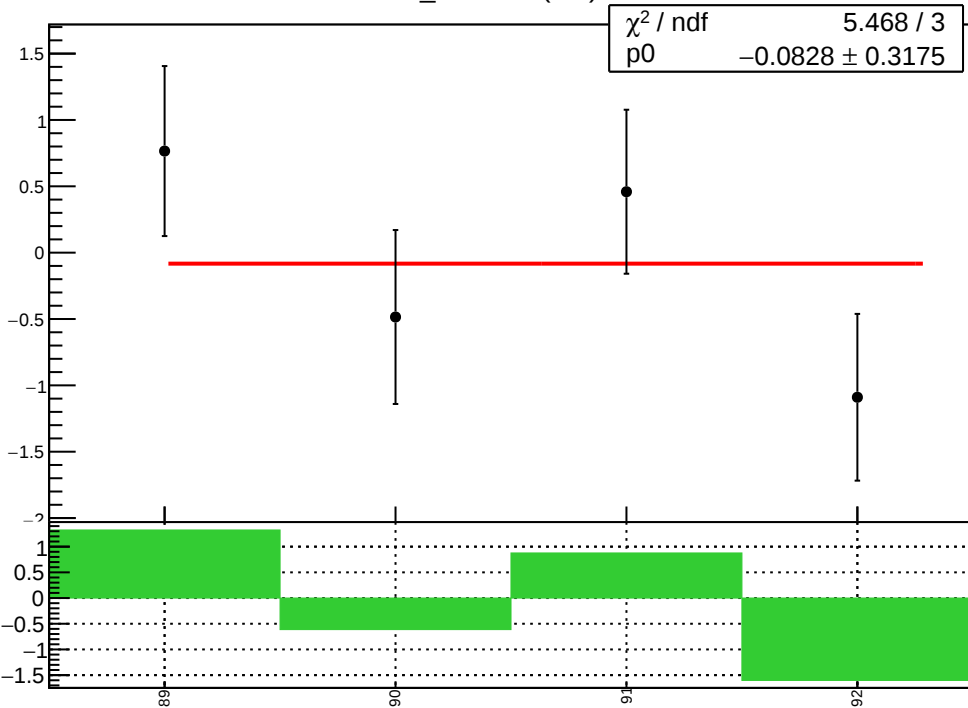
diff_evMon8 (nm)
