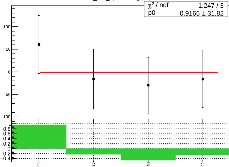
corr_usr_bpm4aY (ppb)
