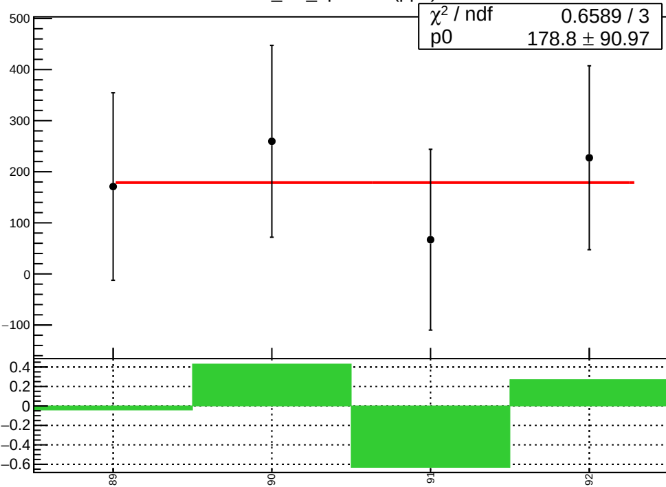
corr_usl_bpm16X (ppb)
