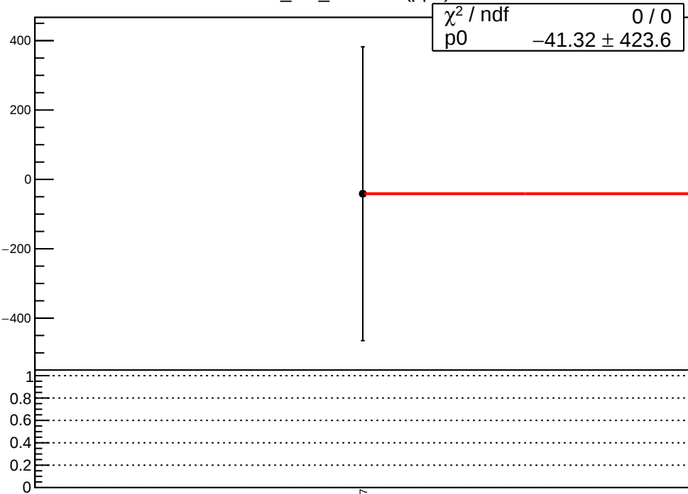
corr_usr_evMon1 (ppb)
