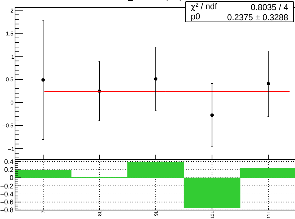
diff_evMon9 (nm)
