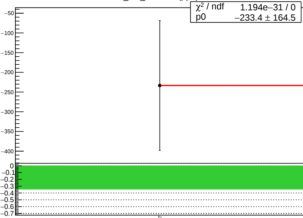
corr_usr_evMon4 (ppb)
