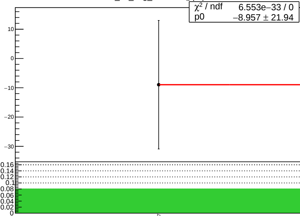
corr_us_avg_evMon5 (ppb)
