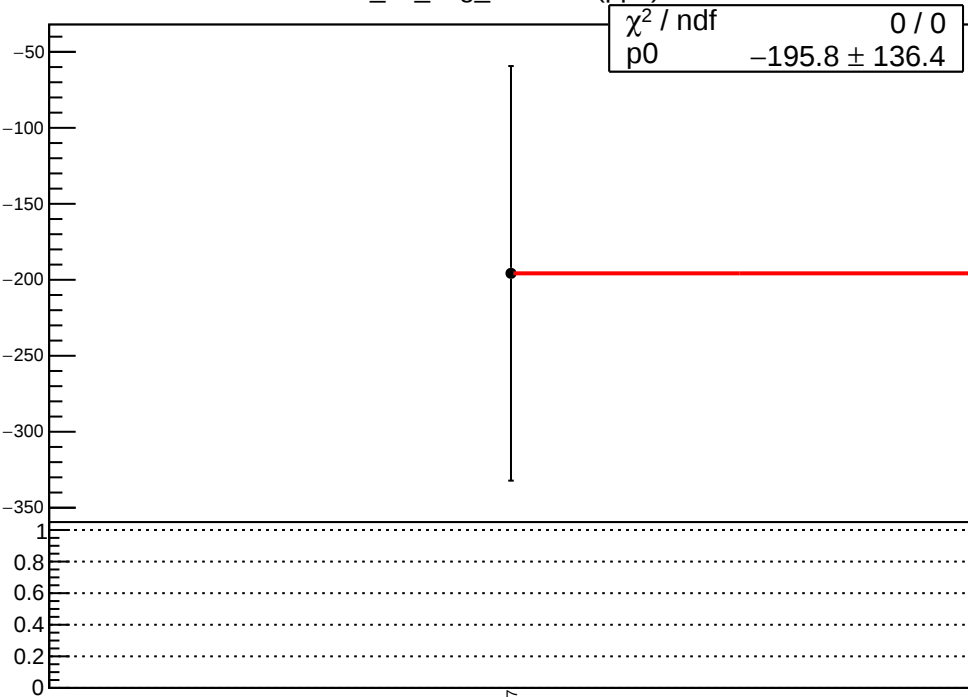
corr_us_avg_evMon4 (ppb)
