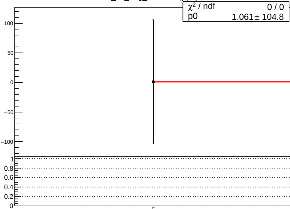
corr_us_avg_evMon3 (ppb)
