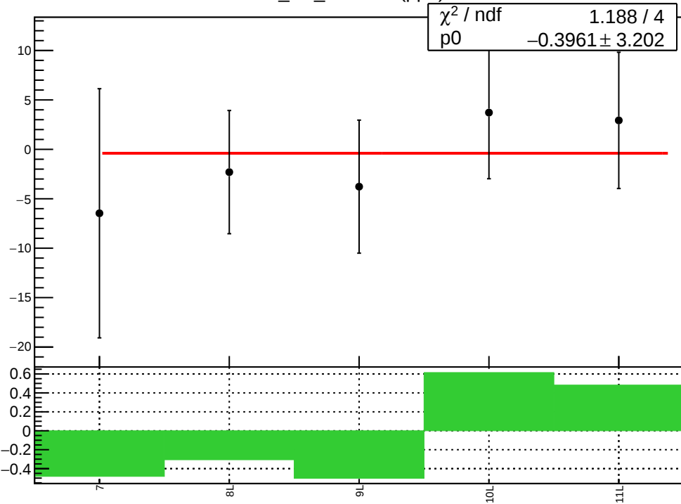
corr_usl_evMon9 (ppb)
