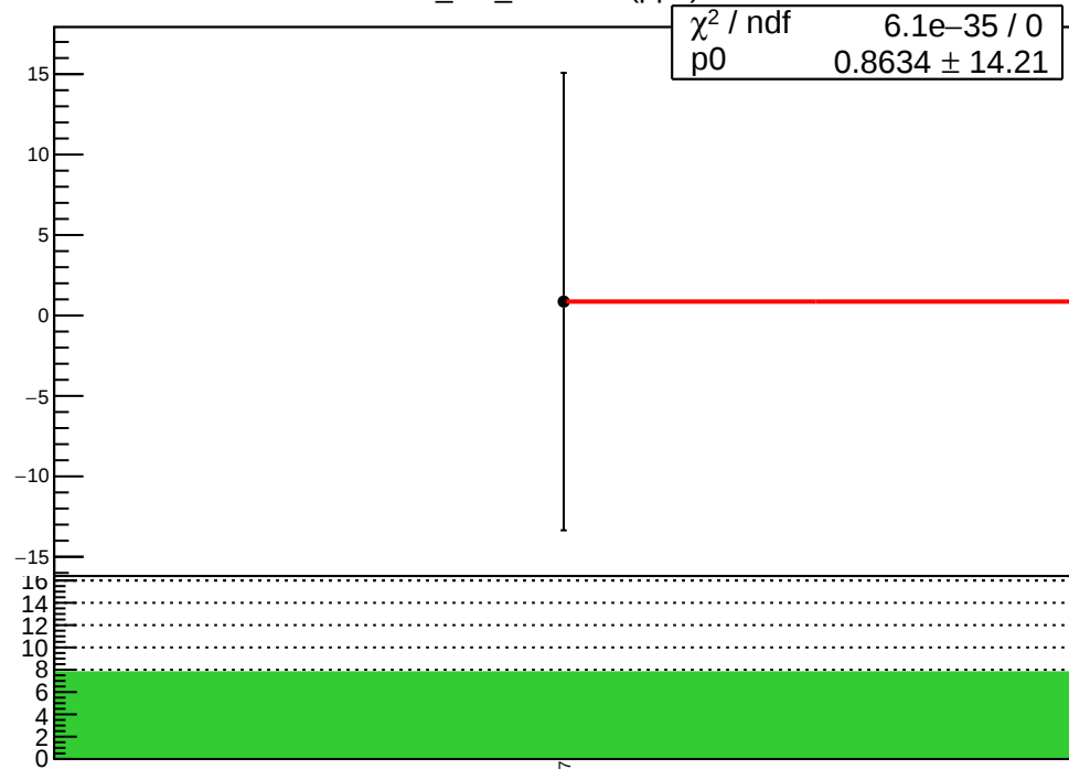
corr_usr_evMon9 (ppb)
