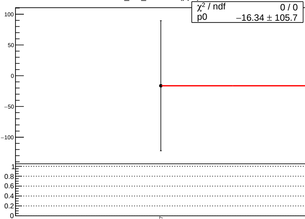
corr_usr_evMon3 (ppb)
