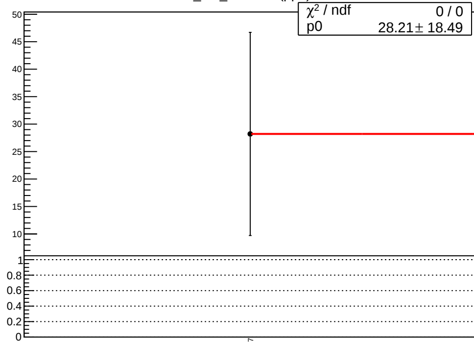
corr_usr_evMon5 (ppb)
