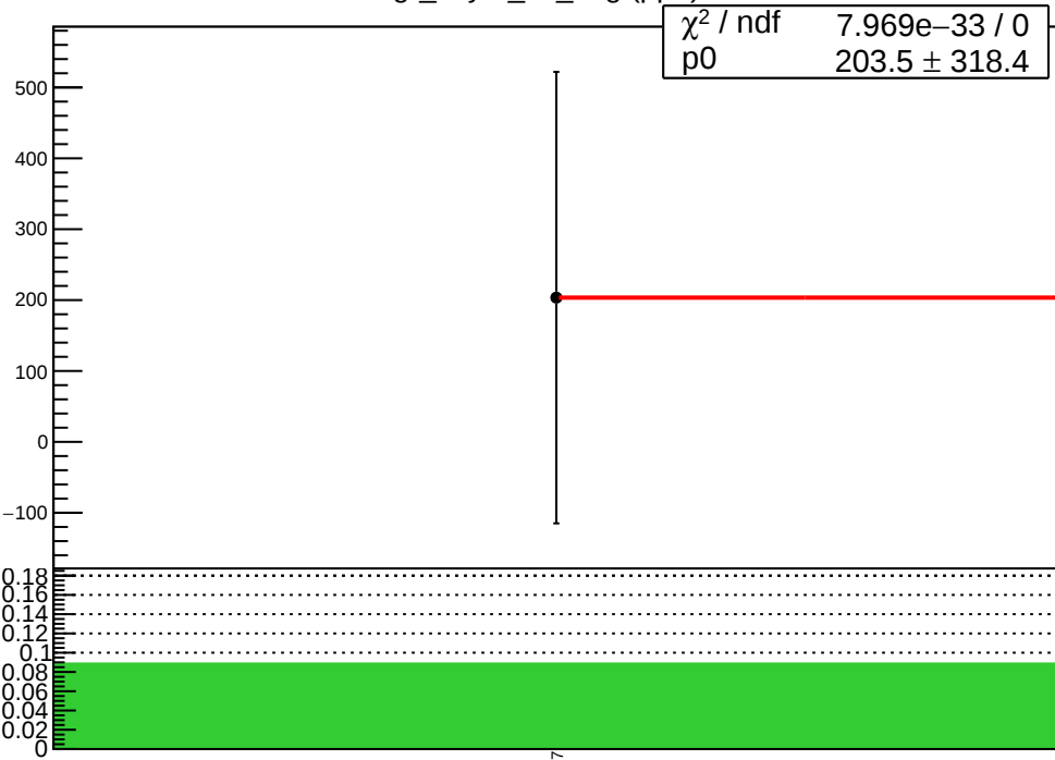
lagr_asym_us_avg (ppb)
