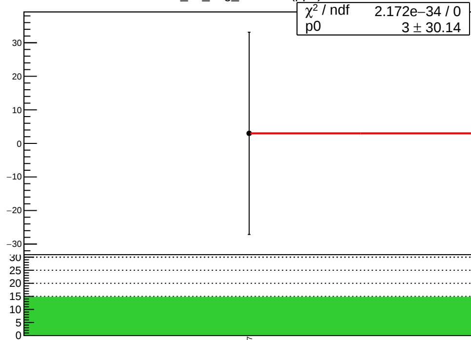
corr_us_avg_evMon6 (ppb)
