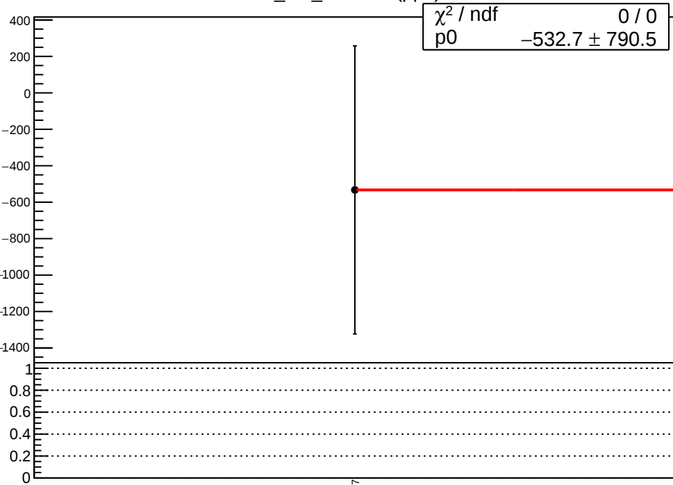
corr_usr_evMon2 (ppb)
