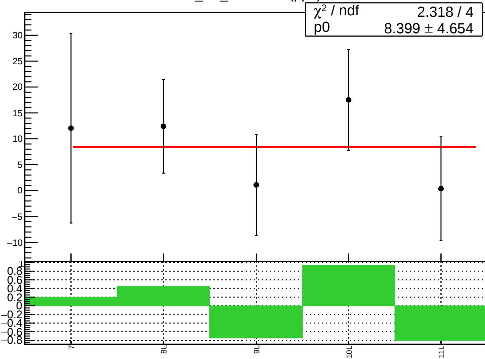
corr_usl_evMon11 (ppb)
