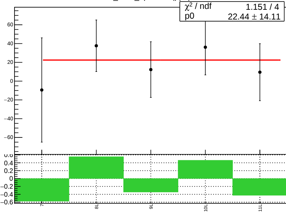
corr_Adet_bpm4aX (ppb)
