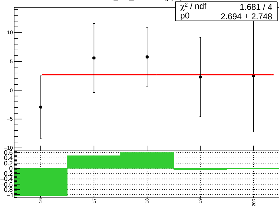
corr_usr_evMon9 (ppb)
