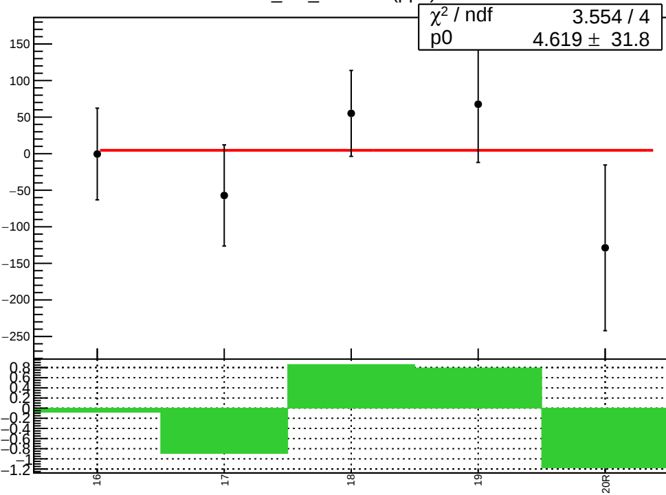
corr_usr_evMon4 (ppb)
