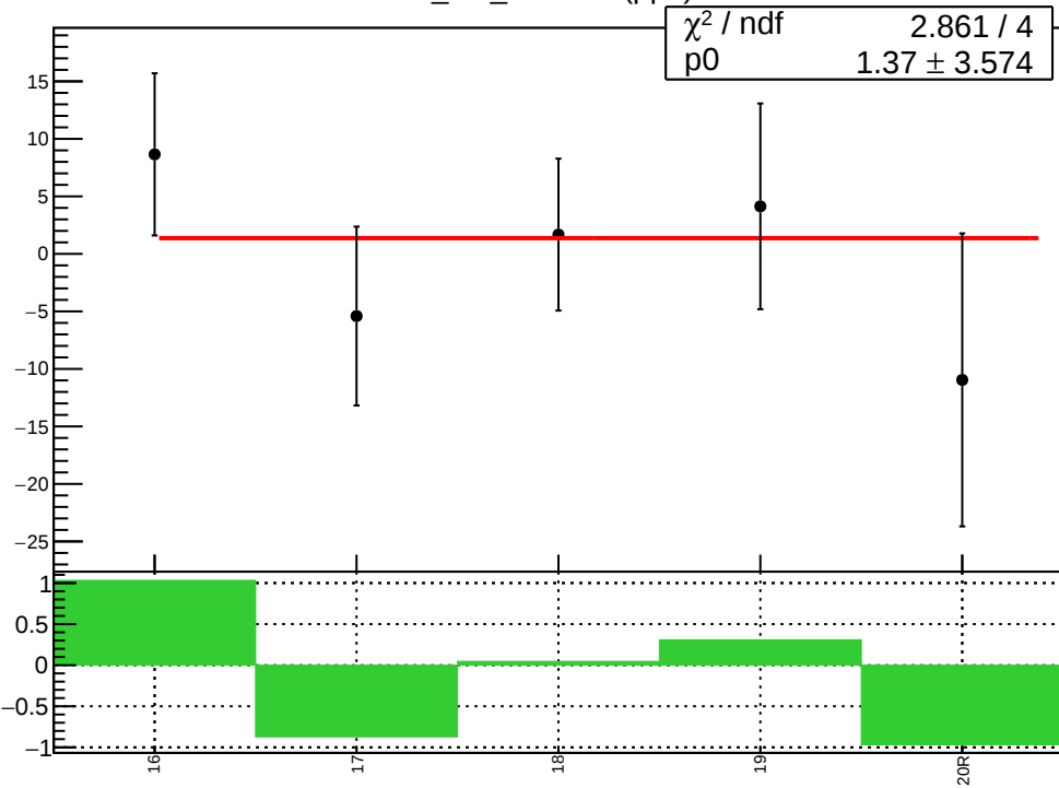
corr_usr_evMon5 (ppb)
