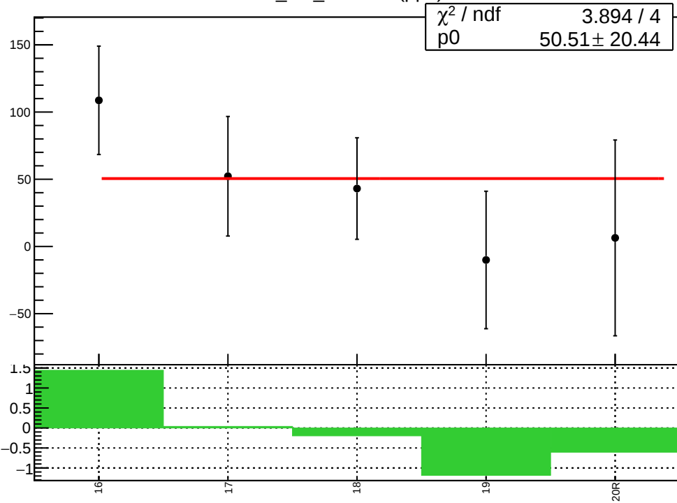
corr_usr_evMon3 (ppb)
