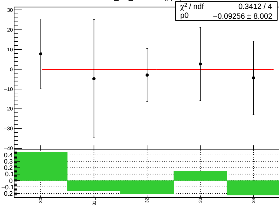
corr_usl_evMon6 (ppb)
