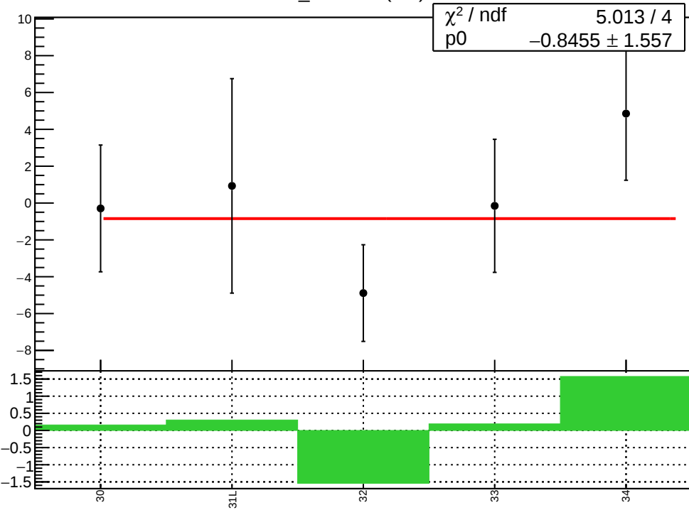
diff_evMon4 (nm)
