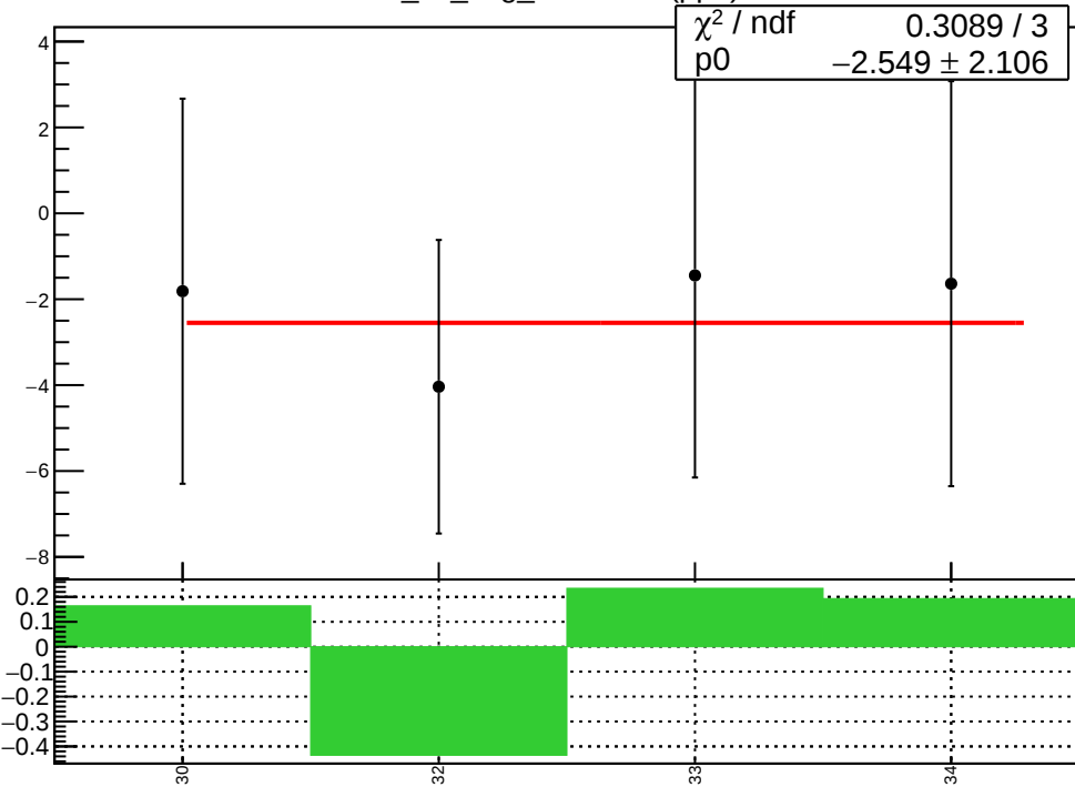
corr_us_avg_evMon10 (ppb)
