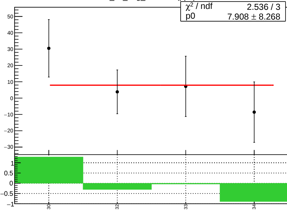
corr_us_avg_evMon7 (ppb)
