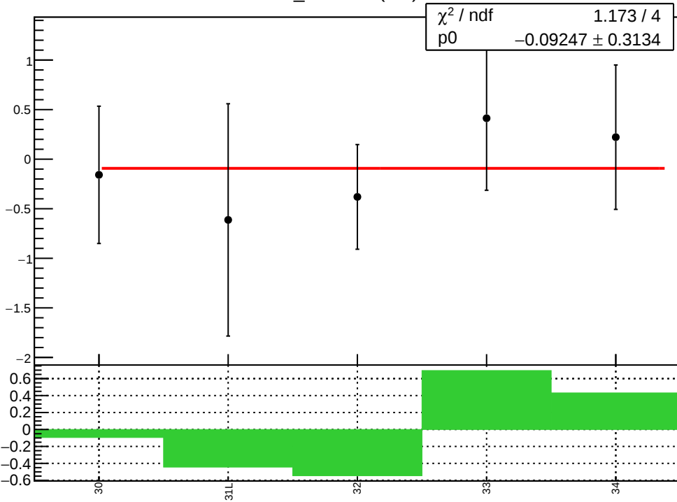
diff_evMon9 (nm)
