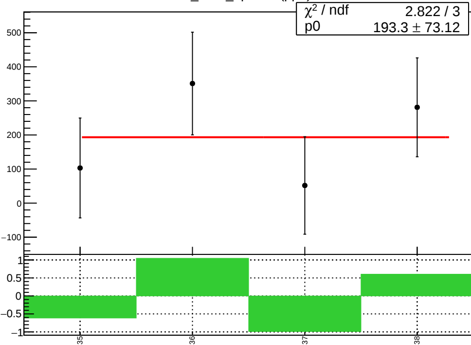
corr_Adet_bpm1X (ppb)
