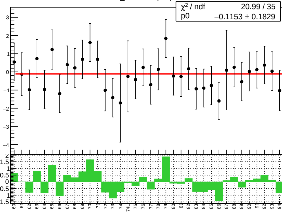
diff_evMon7 (nm)
