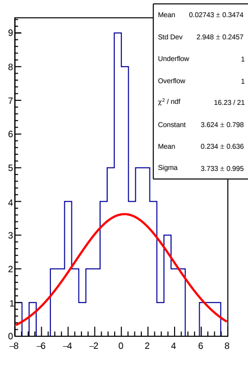
1D pull distribution
