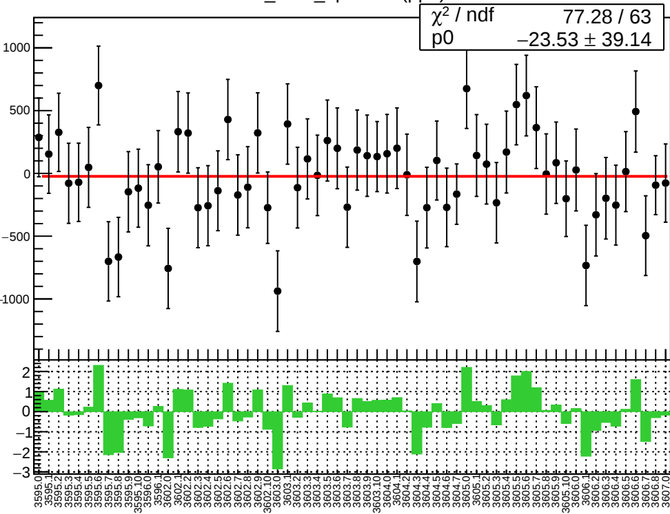
corr_Adet_bpm12Y (ppb)
